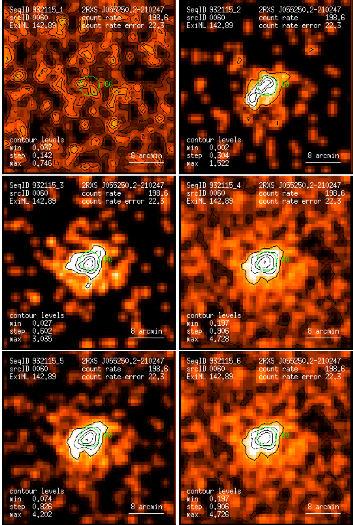
Figure 60: RASS 932115: detection 0060: band rate images, Gaussian filter: (1) PSPC channels 11 – 41, (2) 52 – 90, (3) 91 – 201, (4) 11 – 235, (5) 52 – 201, (6) 11 – 201. Broad band rates in counts/ks. Band rate contour levels in counts/ks/arcmin 2 .
