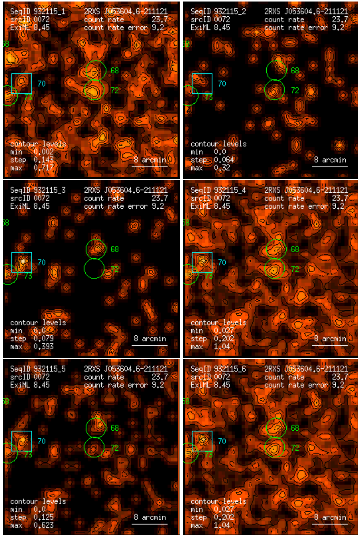
Figure 72: RASS 932115: detection 0072: band rate images, Gaussian filter: (1) PSPC channels 11 – 41, (2) 52 – 90, (3) 91 – 201, (4) 11 – 235, (5) 52 – 201, (6) 11 – 201. Broad band rates in counts/ks. Band rate contour levels in counts/ks/arcmin 2 .
