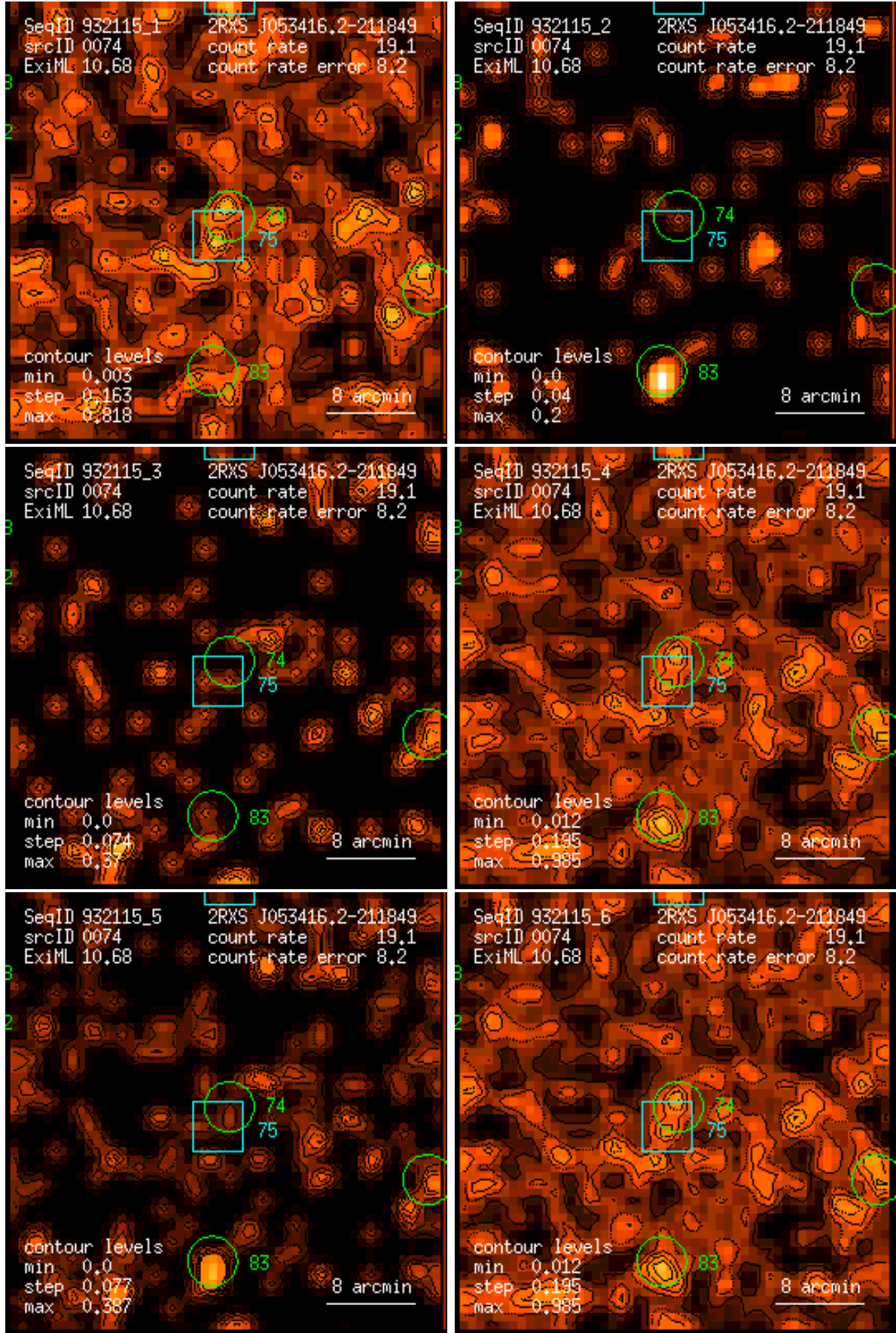
Figure 74: RASS 932115: detection 0074: band rate images, Gaussian filter: (1) PSPC channels 11 – 41, (2) 52 – 90, (3) 91 – 201, (4) 11 – 235, (5) 52 – 201, (6) 11 – 201. Broad band rates in counts/ks. Band rate contour levels in counts/ks/arcmin 2 .
