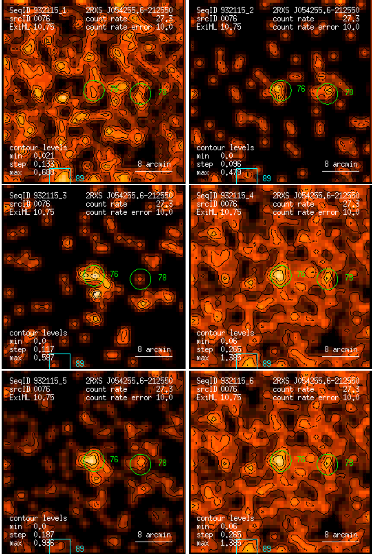
Figure 76: RASS 932115: detection 0076: band rate images, Gaussian filter: (1) PSPC channels 11 – 41, (2) 52 – 90, (3) 91 – 201, (4) 11 – 235, (5) 52 – 201, (6) 11 – 201. Broad band rates in counts/ks. Band rate contour levels in counts/ks/arcmin 2 .
