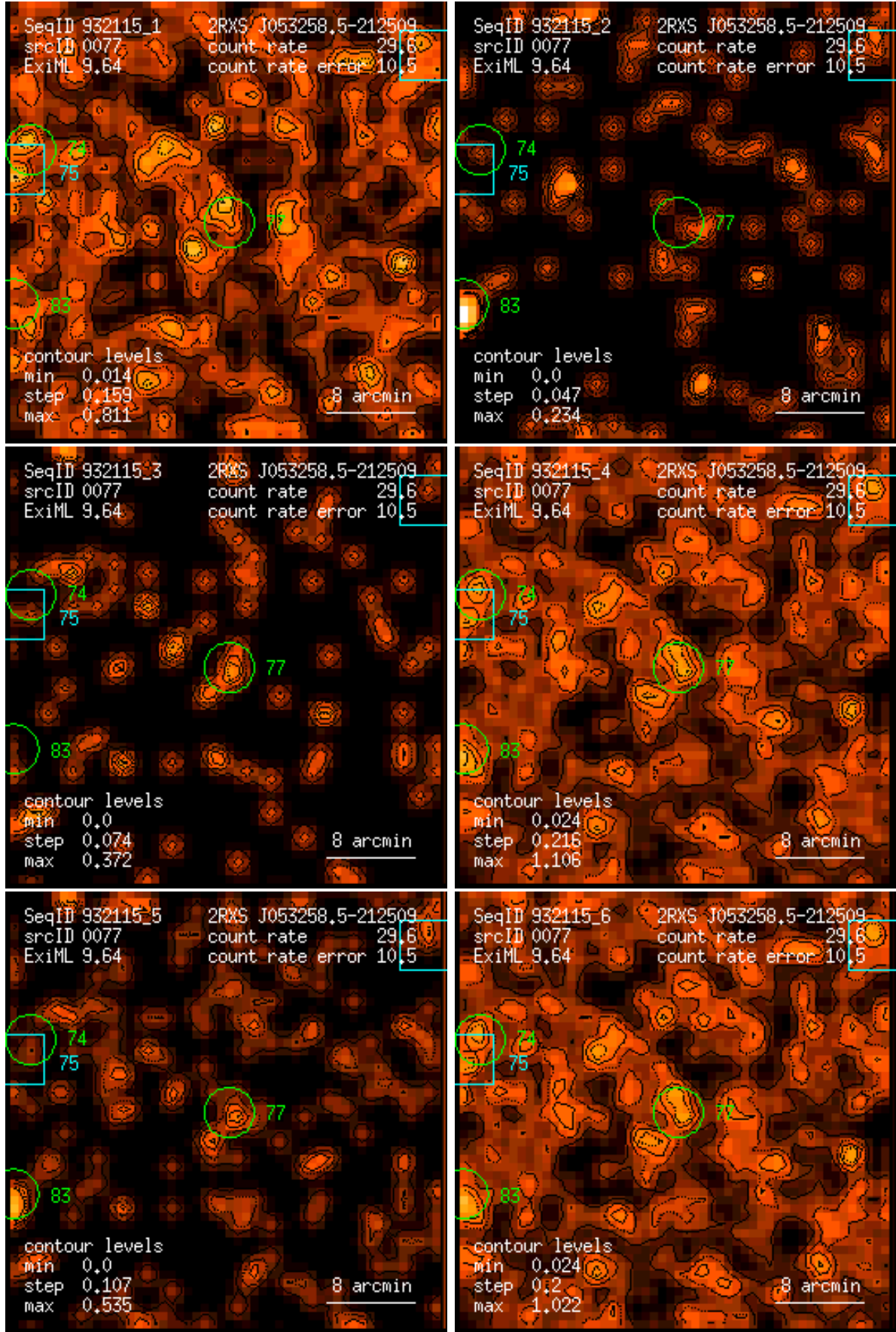
Figure 77: RASS 932115: detection 0077: band rate images, Gaussian filter: (1) PSPC channels 11 – 41, (2) 52 – 90, (3) 91 – 201, (4) 11 – 235, (5) 52 – 201, (6) 11 – 201. Broad band rates in counts/ks. Band rate contour levels in counts/ks/arcmin 2 .
