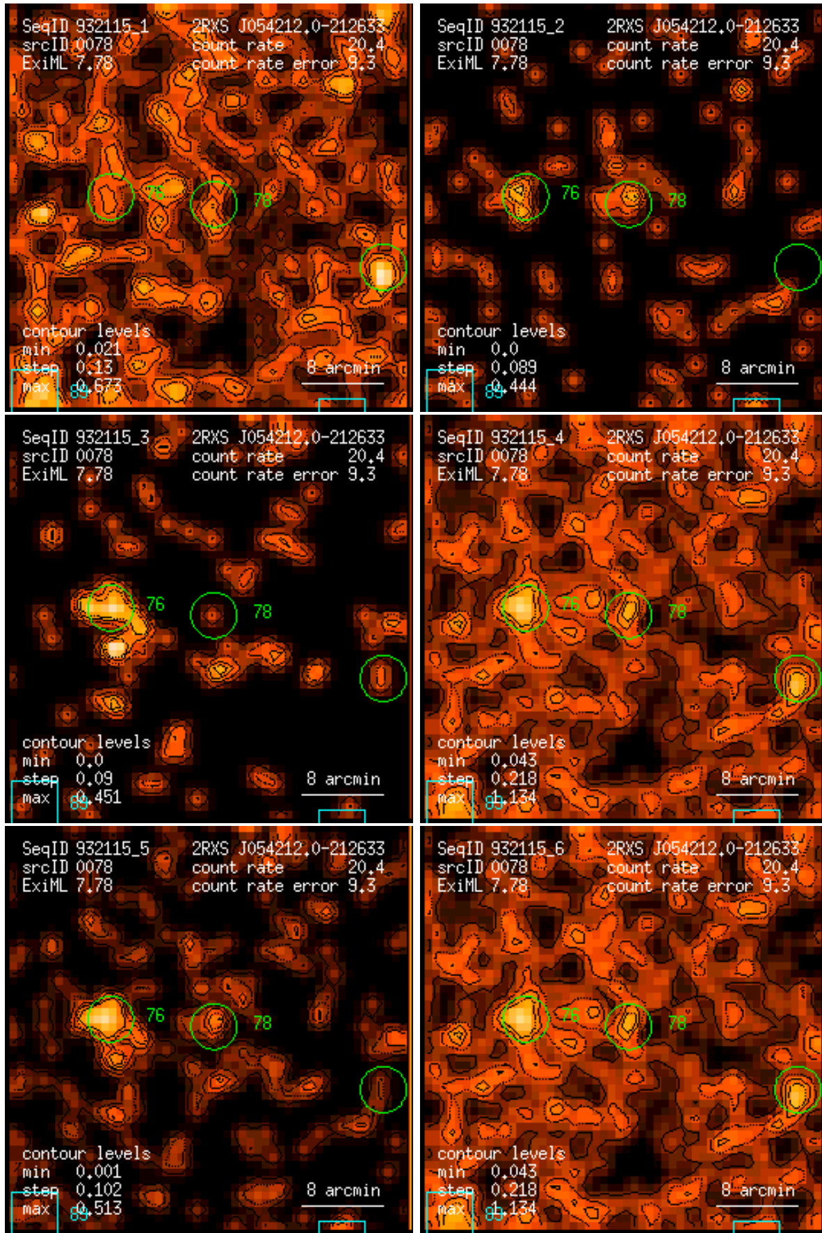
Figure 78: RASS 932115: detection 0078: band rate images, Gaussian filter: (1) PSPC channels 11 – 41, (2) 52 – 90, (3) 91 – 201, (4) 11 – 235, (5) 52 – 201, (6) 11 – 201. Broad band rates in counts/ks. Band rate contour levels in counts/ks/arcmin 2 .
