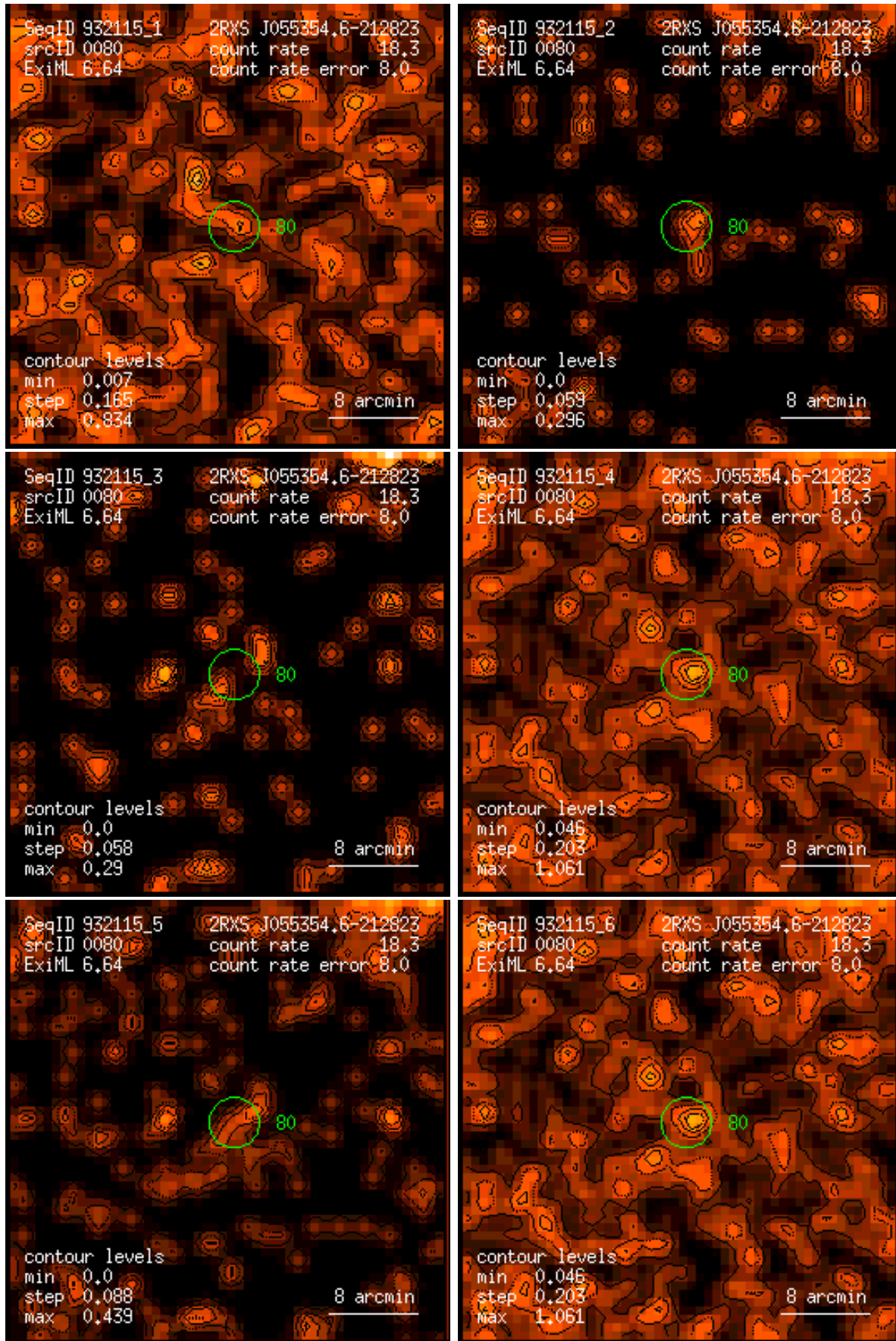
Figure 80: RASS 932115: detection 0080: band rate images, Gaussian filter: (1) PSPC channels 11 – 41, (2) 52 – 90, (3) 91 – 201, (4) 11 – 235, (5) 52 – 201, (6) 11 – 201. Broad band rates in counts/ks. Band rate contour levels in counts/ks/arcmin 2 .
