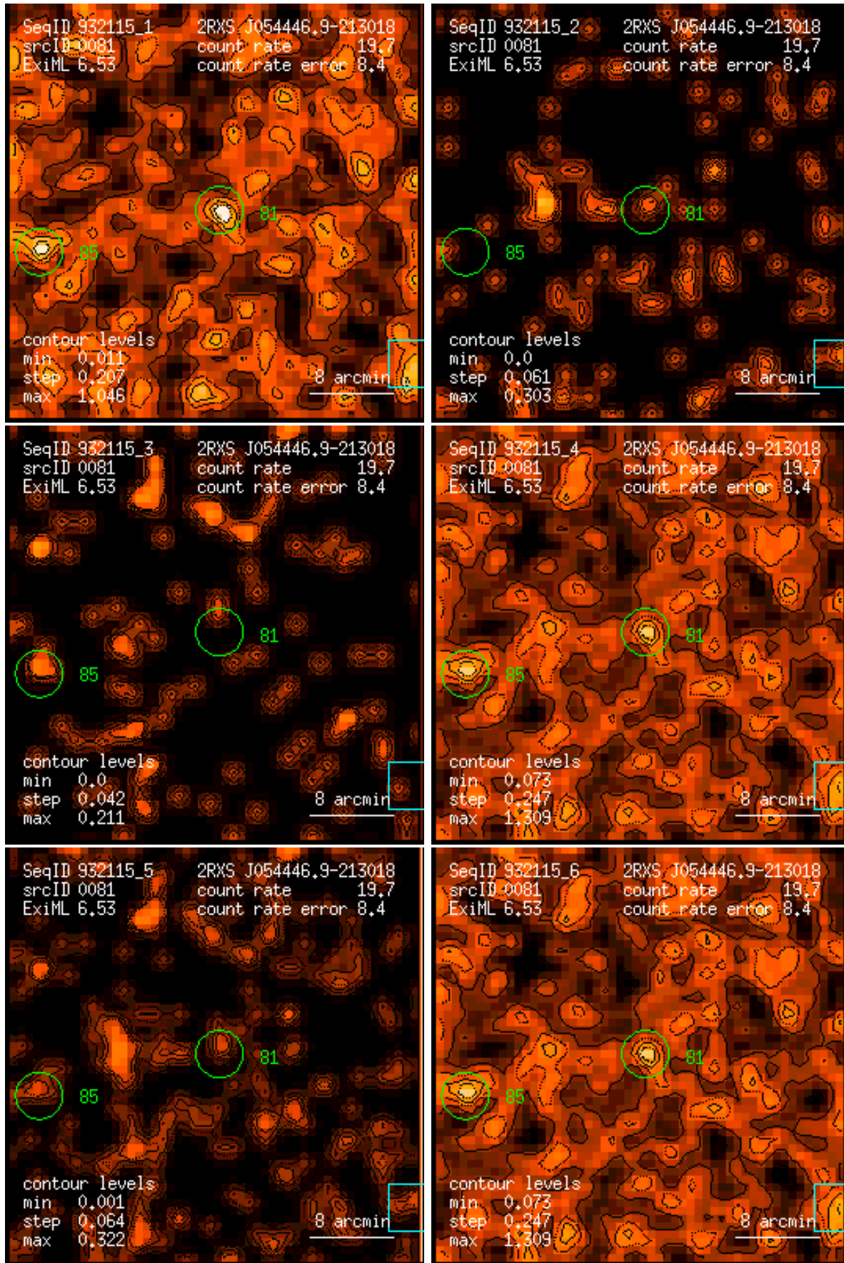
Figure 81: RASS 932115: detection 0081: band rate images, Gaussian filter: (1) PSPC channels 11 – 41, (2) 52 – 90, (3) 91 – 201, (4) 11 – 235, (5) 52 – 201, (6) 11 – 201. Broad band rates in counts/ks. Band rate contour levels in counts/ks/arcmin 2 .
