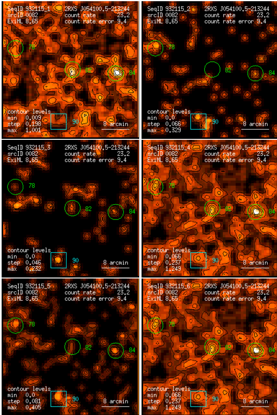
Figure 82: RASS 932115: detection 0082: band rate images, Gaussian filter: (1) PSPC channels 11 – 41, (2) 52 – 90, (3) 91 – 201, (4) 11 – 235, (5) 52 – 201, (6) 11 – 201. Broad band rates in counts/ks. Band rate contour levels in counts/ks/arcmin 2 .
