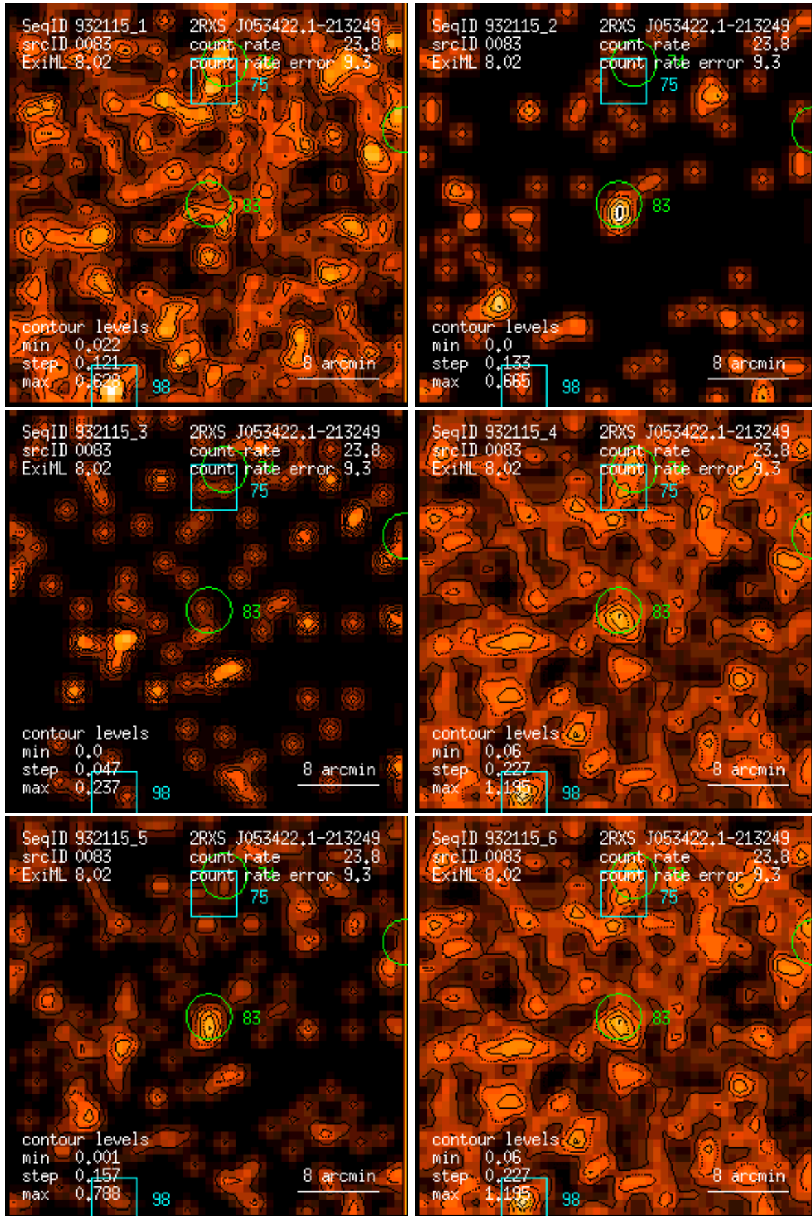
Figure 83: RASS 932115: detection 0083: band rate images, Gaussian filter: (1) PSPC channels 11 – 41, (2) 52 – 90, (3) 91 – 201, (4) 11 – 235, (5) 52 – 201, (6) 11 – 201. Broad band rates in counts/ks. Band rate contour levels in counts/ks/arcmin 2 .
