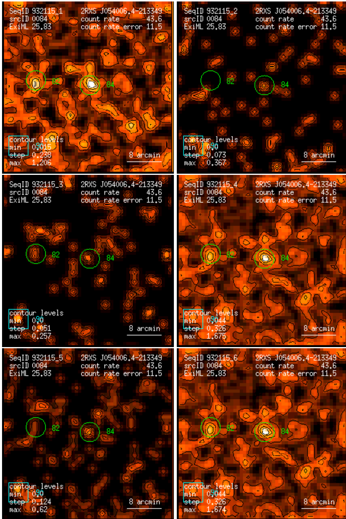
Figure 84: RASS 932115: detection 0084: band rate images, Gaussian filter: (1) PSPC channels 11 – 41, (2) 52 – 90, (3) 91 – 201, (4) 11 – 235, (5) 52 – 201, (6) 11 – 201. Broad band rates in counts/ks. Band rate contour levels in counts/ks/arcmin 2 .
