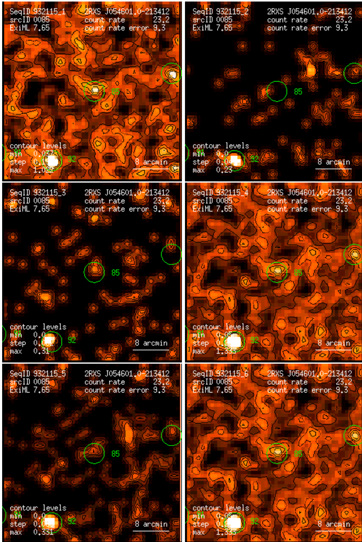
Figure 85: RASS 932115: detection 0085: band rate images, Gaussian filter: (1) PSPC channels 11 – 41, (2) 52 – 90, (3) 91 – 201, (4) 11 – 235, (5) 52 – 201, (6) 11 – 201. Broad band rates in counts/ks. Band rate contour levels in counts/ks/arcmin 2 .
