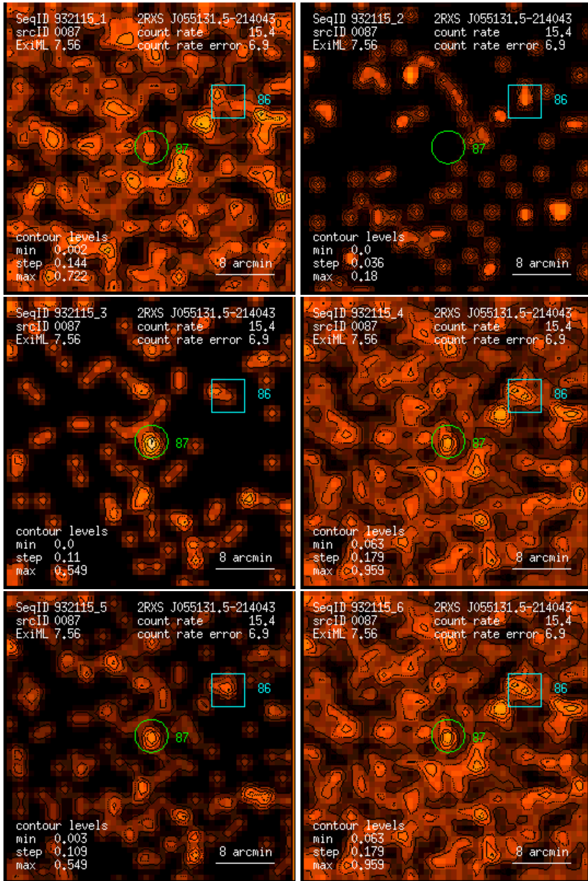
Figure 87: RASS 932115: detection 0087: band rate images, Gaussian filter: (1) PSPC channels 11 – 41, (2) 52 – 90, (3) 91 – 201, (4) 11 – 235, (5) 52 – 201, (6) 11 – 201. Broad band rates in counts/ks. Band rate contour levels in counts/ks/arcmin 2 .
