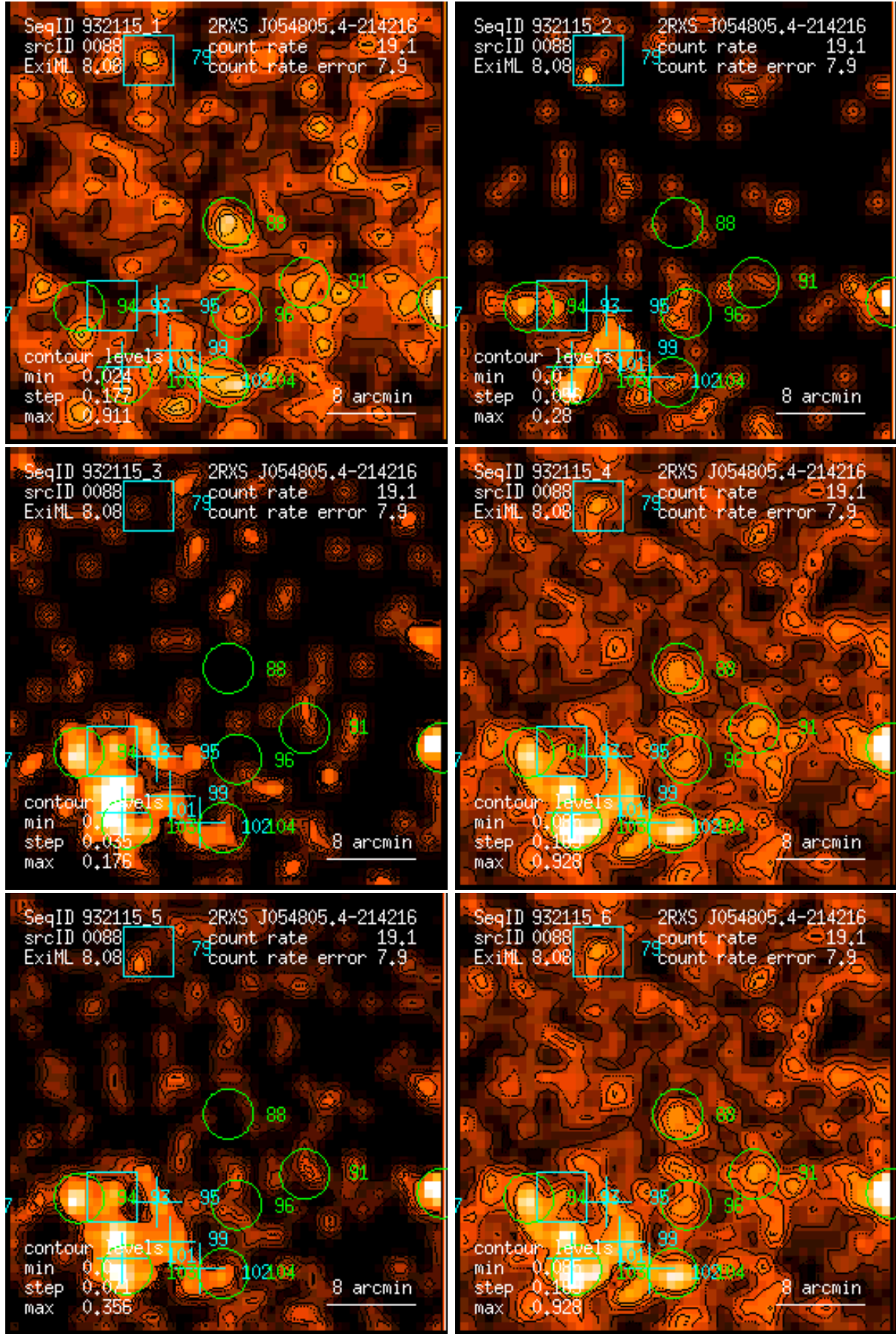
Figure 88: RASS 932115: detection 0088: band rate images, Gaussian filter: (1) PSPC channels 11 – 41, (2) 52 – 90, (3) 91 – 201, (4) 11 – 235, (5) 52 – 201, (6) 11 – 201. Broad band rates in counts/ks. Band rate contour levels in counts/ks/arcmin 2 .
