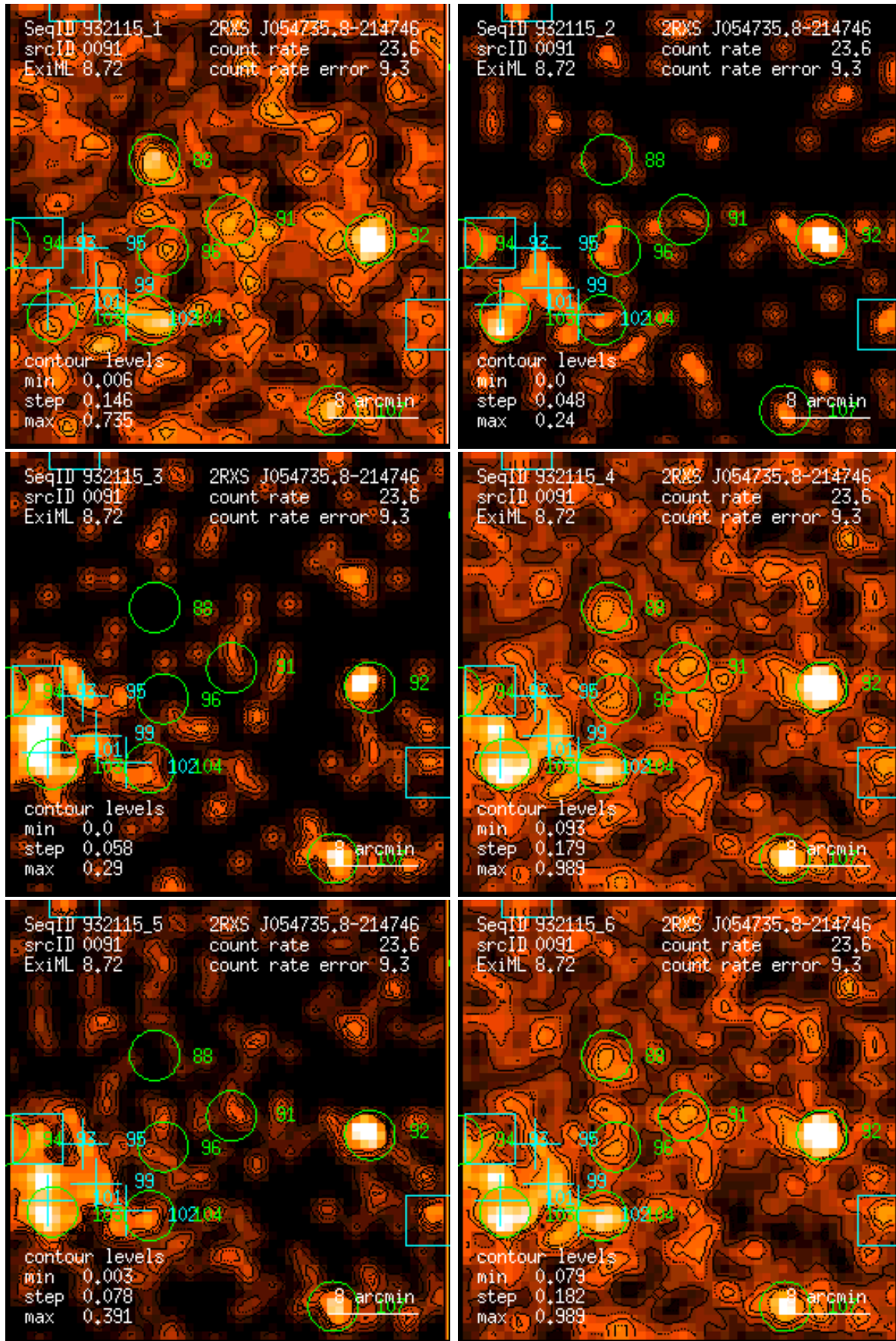
Figure 91: RASS 932115: detection 0091: band rate images, Gaussian filter: (1) PSPC channels 11 – 41, (2) 52 – 90, (3) 91 – 201, (4) 11 – 235, (5) 52 – 201, (6) 11 – 201. Broad band rates in counts/ks. Band rate contour levels in counts/ks/arcmin 2 .
