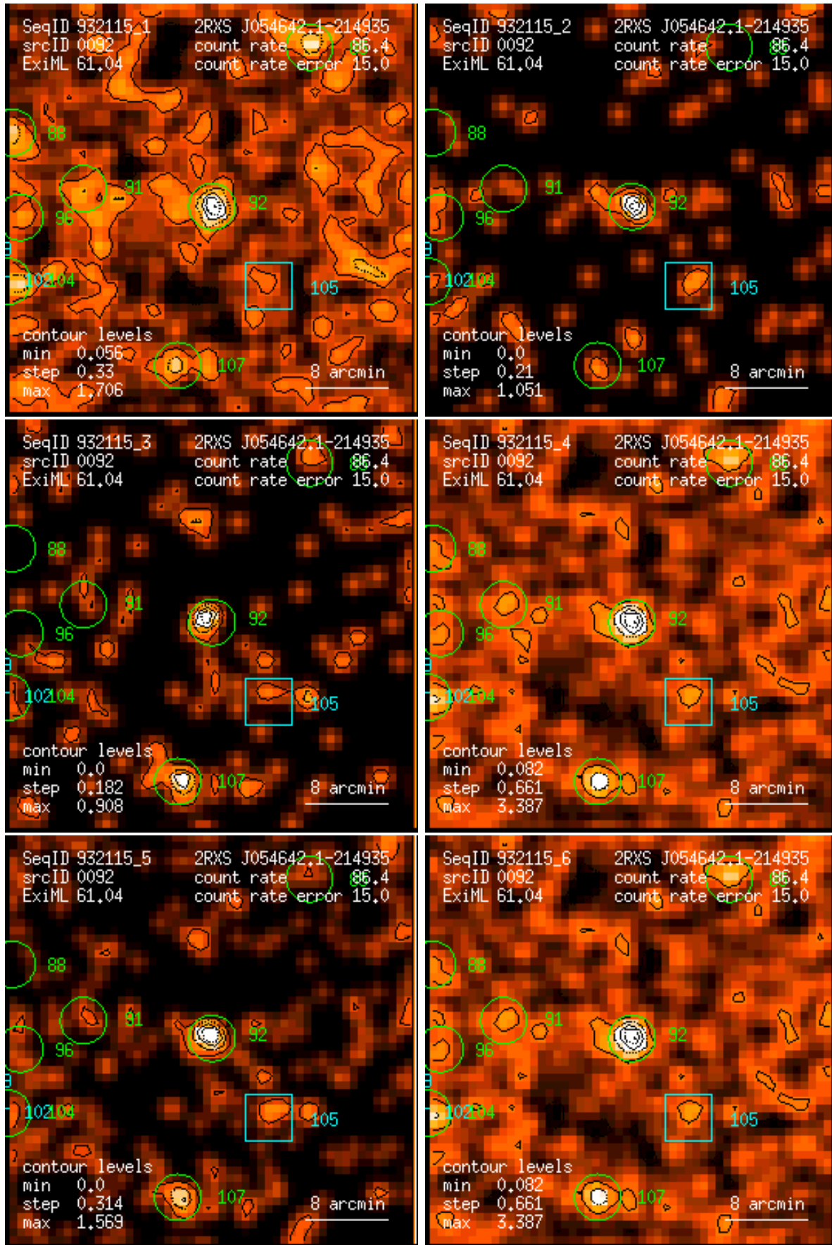
Figure 92: RASS 932115: detection 0092: band rate images, Gaussian filter: (1) PSPC channels 11 – 41, (2) 52 – 90, (3) 91 – 201, (4) 11 – 235, (5) 52 – 201, (6) 11 – 201. Broad band rates in counts/ks. Band rate contour levels in counts/ks/arcmin 2 .
