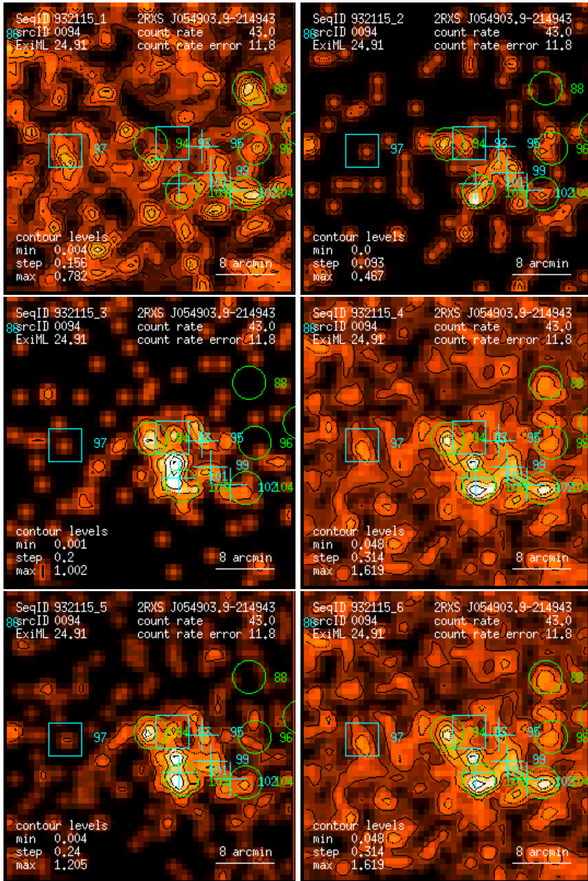
Figure 94: RASS 932115: detection 0094: band rate images, Gaussian filter: (1) PSPC channels 11 – 41, (2) 52 – 90, (3) 91 – 201, (4) 11 – 235, (5) 52 – 201, (6) 11 – 201. Broad band rates in counts/ks. Band rate contour levels in counts/ks/arcmin 2 .
