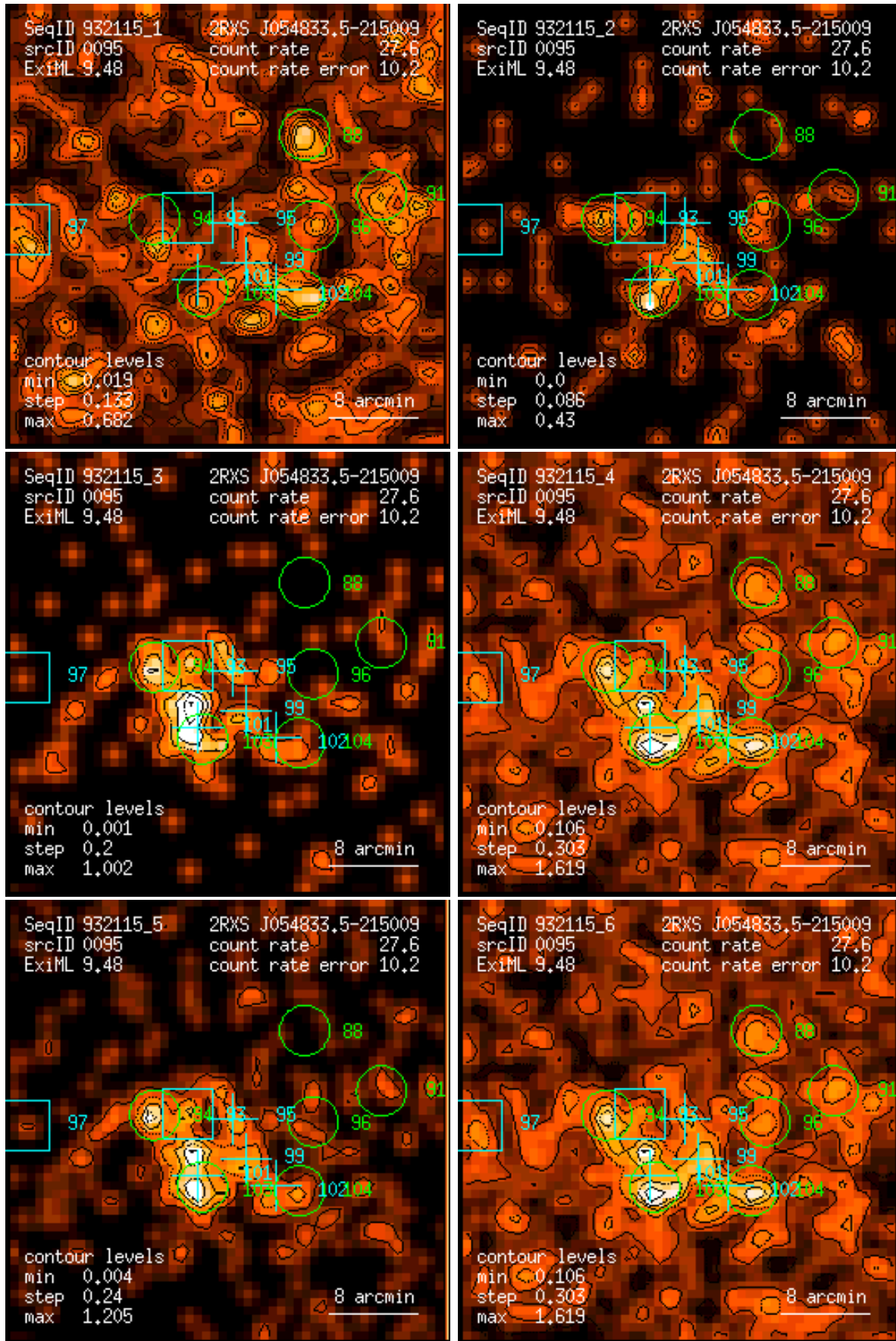
Figure 95: RASS 932115: detection 0095: band rate images, Gaussian filter: (1) PSPC channels 11 – 41, (2) 52 – 90, (3) 91 – 201, (4) 11 – 235, (5) 52 – 201, (6) 11 – 201. Broad band rates in counts/ks. Band rate contour levels in counts/ks/arcmin 2 .
