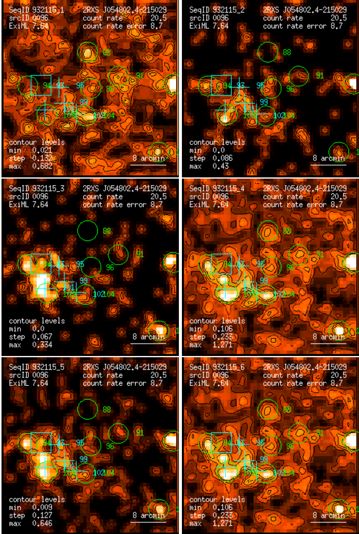
Figure 96: RASS 932115: detection 0096: band rate images, Gaussian filter: (1) PSPC channels 11 – 41, (2) 52 – 90, (3) 91 – 201, (4) 11 – 235, (5) 52 – 201, (6) 11 – 201. Broad band rates in counts/ks. Band rate contour levels in counts/ks/arcmin 2 .
