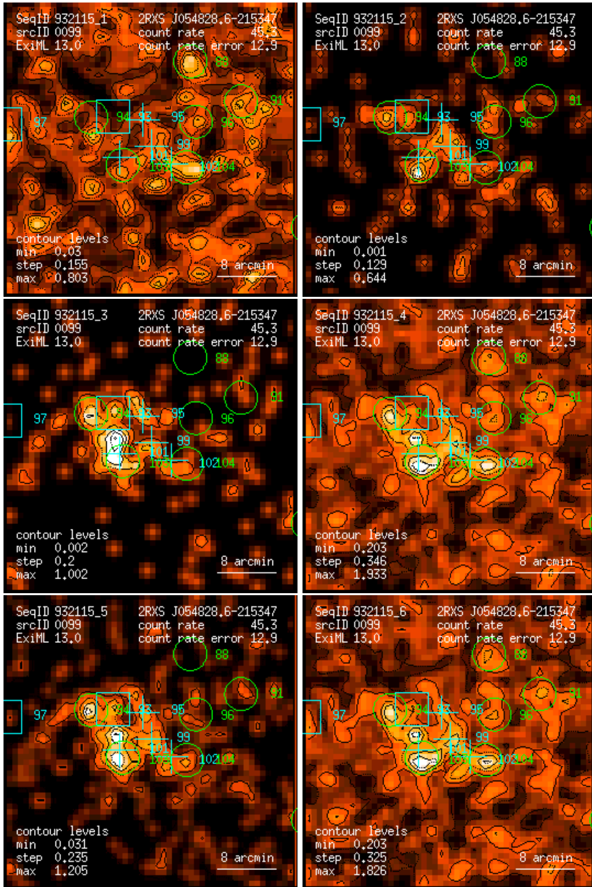
Figure 99: RASS 932115: detection 0099: band rate images, Gaussian filter: (1) PSPC channels 11 – 41, (2) 52 – 90, (3) 91 – 201, (4) 11 – 235, (5) 52 – 201, (6) 11 – 201. Broad band rates in counts/ks. Band rate contour levels in counts/ks/arcmin 2 .
