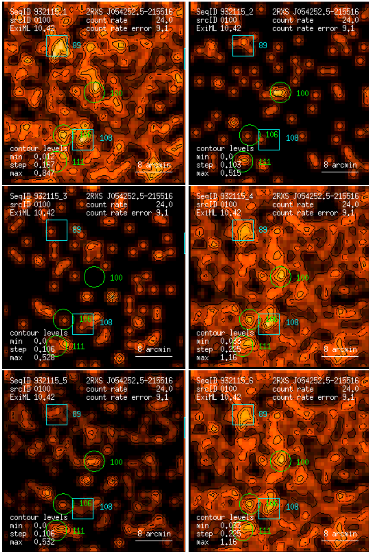
Figure 100: RASS 932115: detection 0100: band rate images, Gaussian filter: (1) PSPC channels 11 – 41, (2) 52 – 90, (3) 91 – 201, (4) 11 – 235, (5) 52 – 201, (6) 11 – 201. Broad band rates in counts/ks. Band rate contour levels in counts/ks/arcmin 2 .
