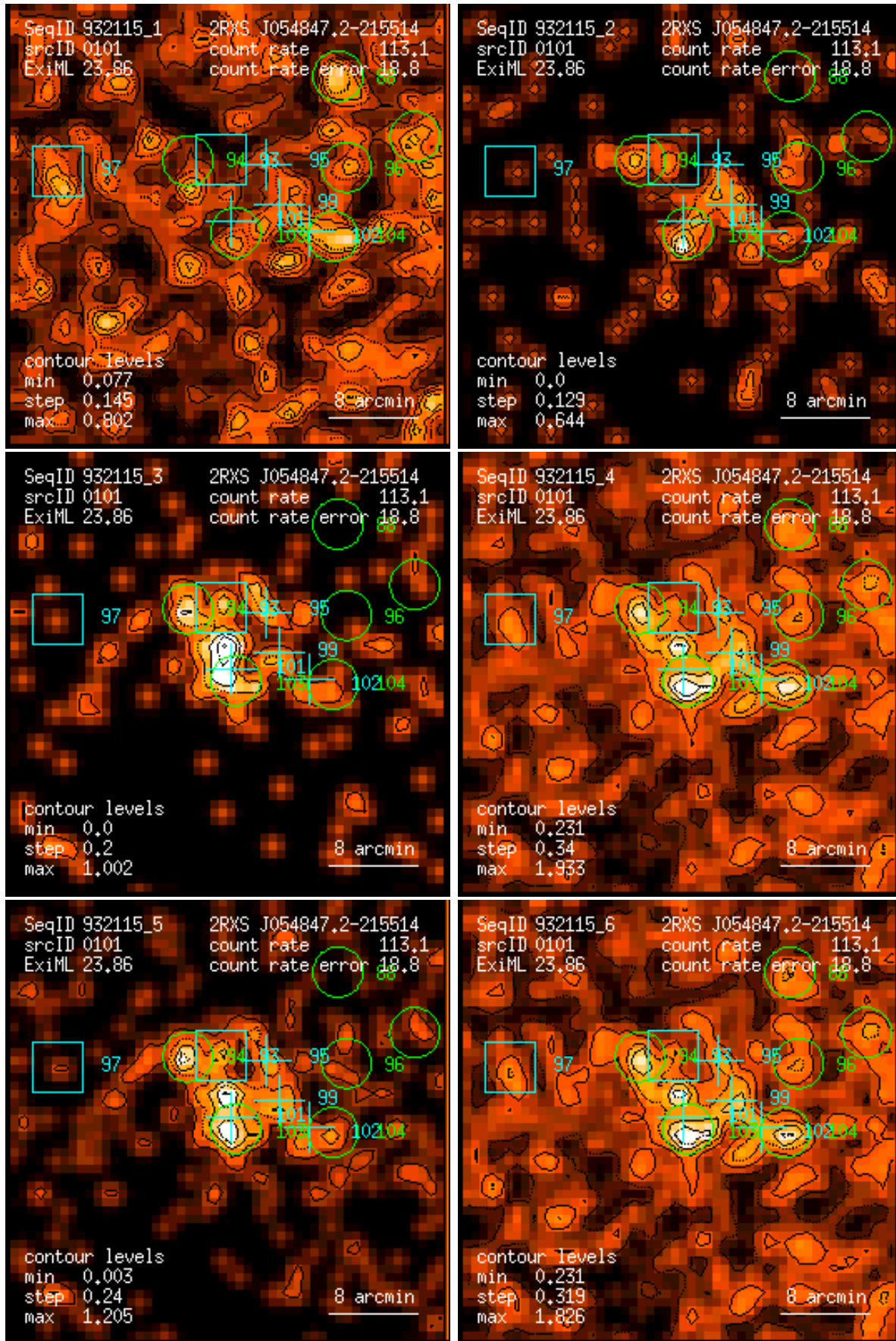
Figure 101: RASS 932115: detection 0101: band rate images, Gaussian filter: (1) PSPC channels 11 – 41, (2) 52 – 90, (3) 91 – 201, (4) 11 – 235, (5) 52 – 201, (6) 11 – 201. Broad band rates in counts/ks. Band rate contour levels in counts/ks/arcmin 2 .
