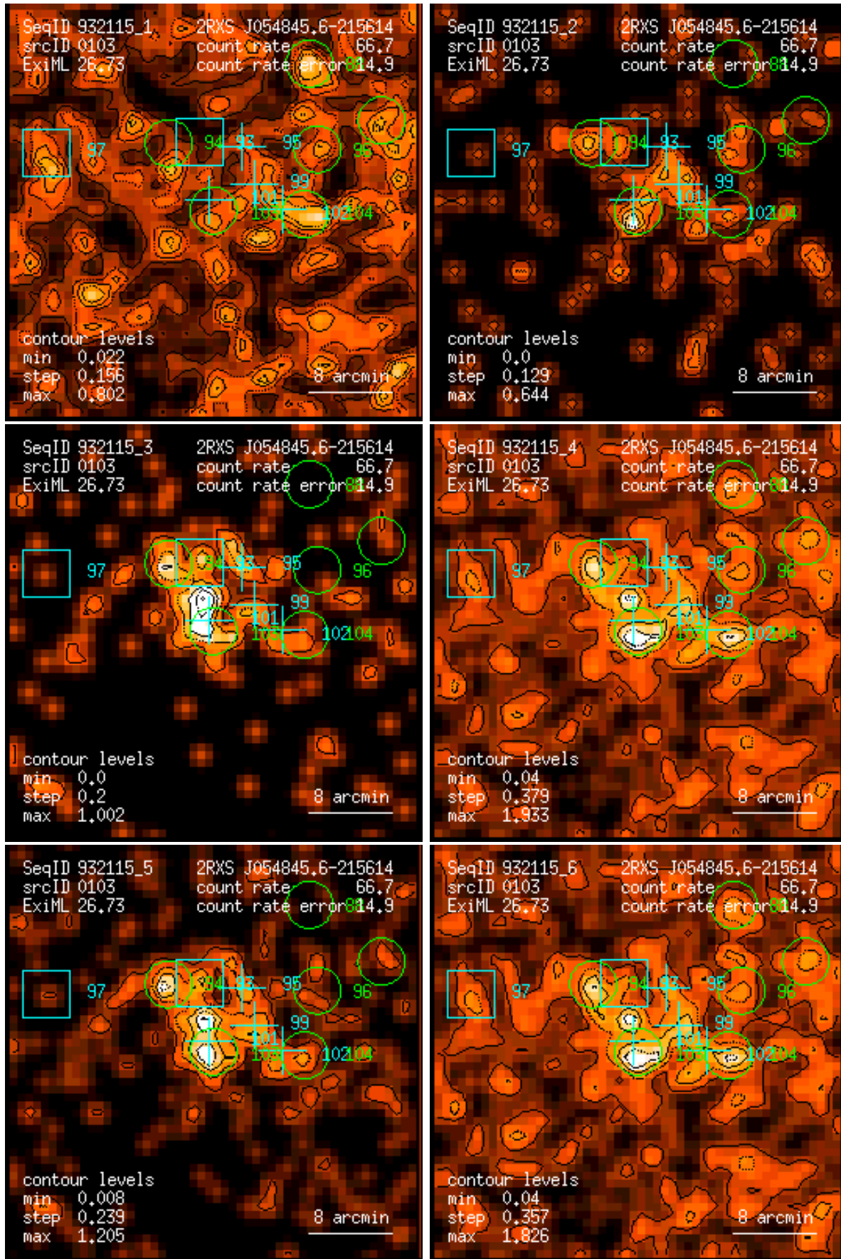
Figure 103: RASS 932115: detection 0103: band rate images, Gaussian filter: (1) PSPC channels 11 – 41, (2) 52 – 90, (3) 91 – 201, (4) 11 – 235, (5) 52 – 201, (6) 11 – 201. Broad band rates in counts/ks. Band rate contour levels in counts/ks/arcmin 2 .
