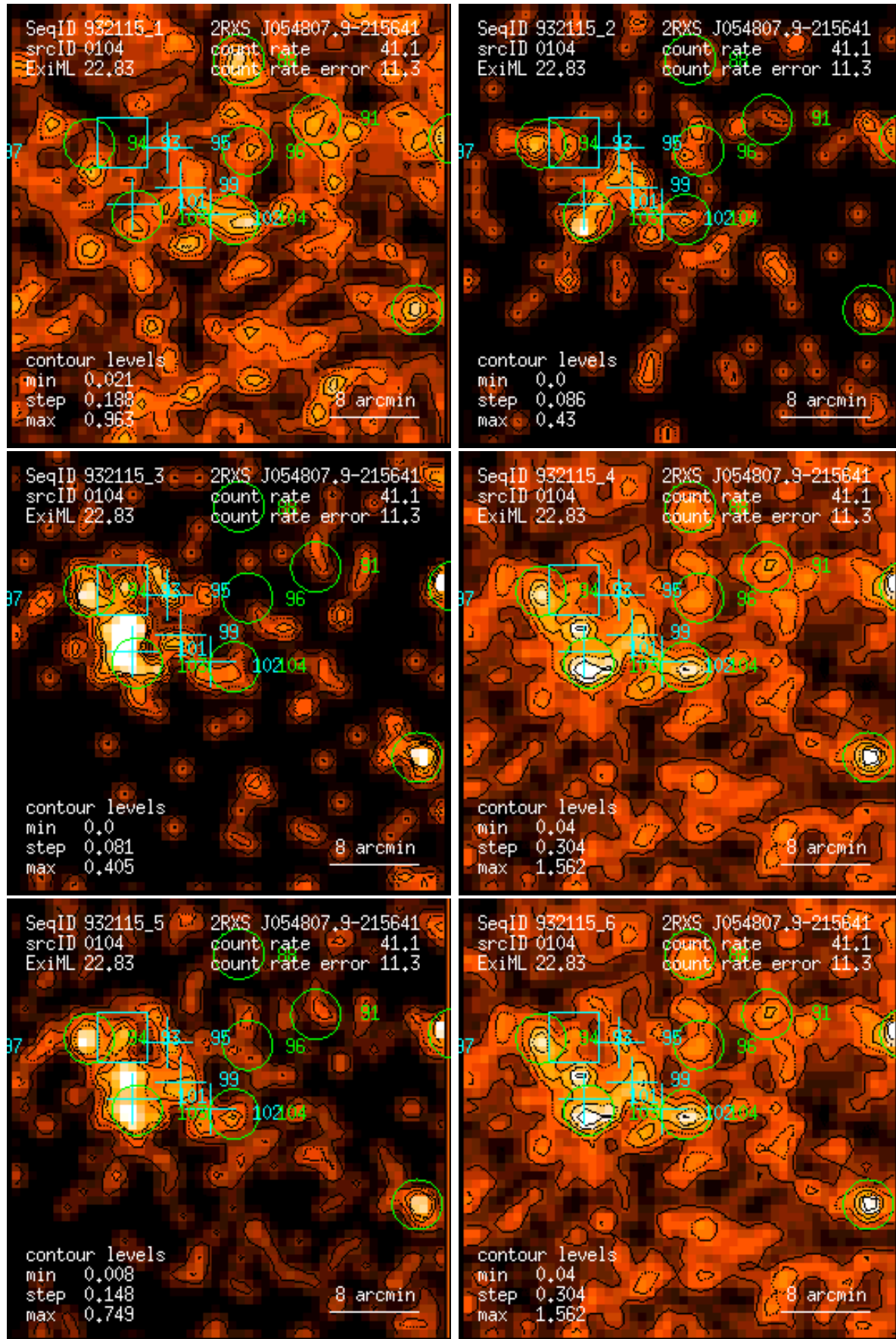
Figure 104: RASS 932115: detection 0104: band rate images, Gaussian filter: (1) PSPC channels 11 – 41, (2) 52 – 90, (3) 91 – 201, (4) 11 – 235, (5) 52 – 201, (6) 11 – 201. Broad band rates in counts/ks. Band rate contour levels in counts/ks/arcmin 2 .
