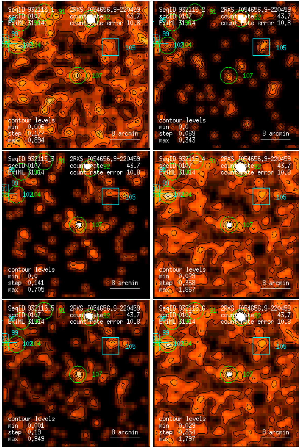
Figure 107: RASS 932115: detection 0107: band rate images, Gaussian filter: (1) PSPC channels 11 – 41, (2) 52 – 90, (3) 91 – 201, (4) 11 – 235, (5) 52 – 201, (6) 11 – 201. Broad band rates in counts/ks. Band rate contour levels in counts/ks/arcmin 2 .
