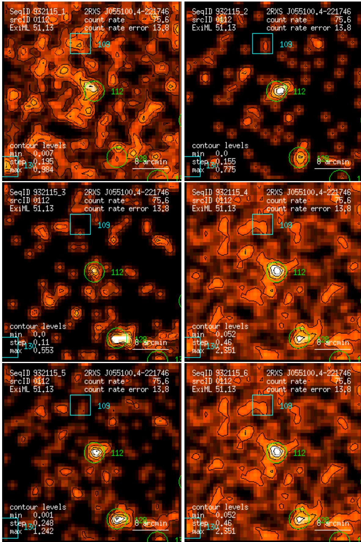
Figure 112: RASS 932115: detection 0112: band rate images, Gaussian filter: (1) PSPC channels 11 – 41, (2) 52 – 90, (3) 91 – 201, (4) 11 – 235, (5) 52 – 201, (6) 11 – 201. Broad band rates in counts/ks. Band rate contour levels in counts/ks/arcmin 2 .
