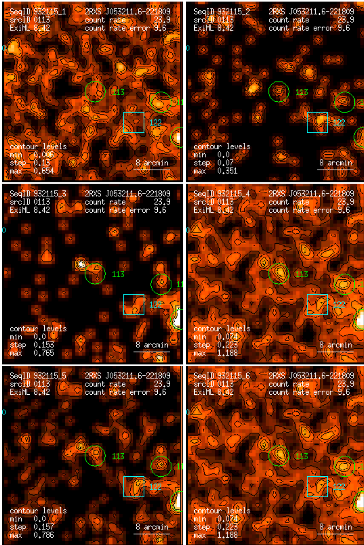
Figure 113: RASS 932115: detection 0113: band rate images, Gaussian filter: (1) PSPC channels 11 – 41, (2) 52 – 90, (3) 91 – 201, (4) 11 – 235, (5) 52 – 201, (6) 11 – 201. Broad band rates in counts/ks. Band rate contour levels in counts/ks/arcmin 2 .
