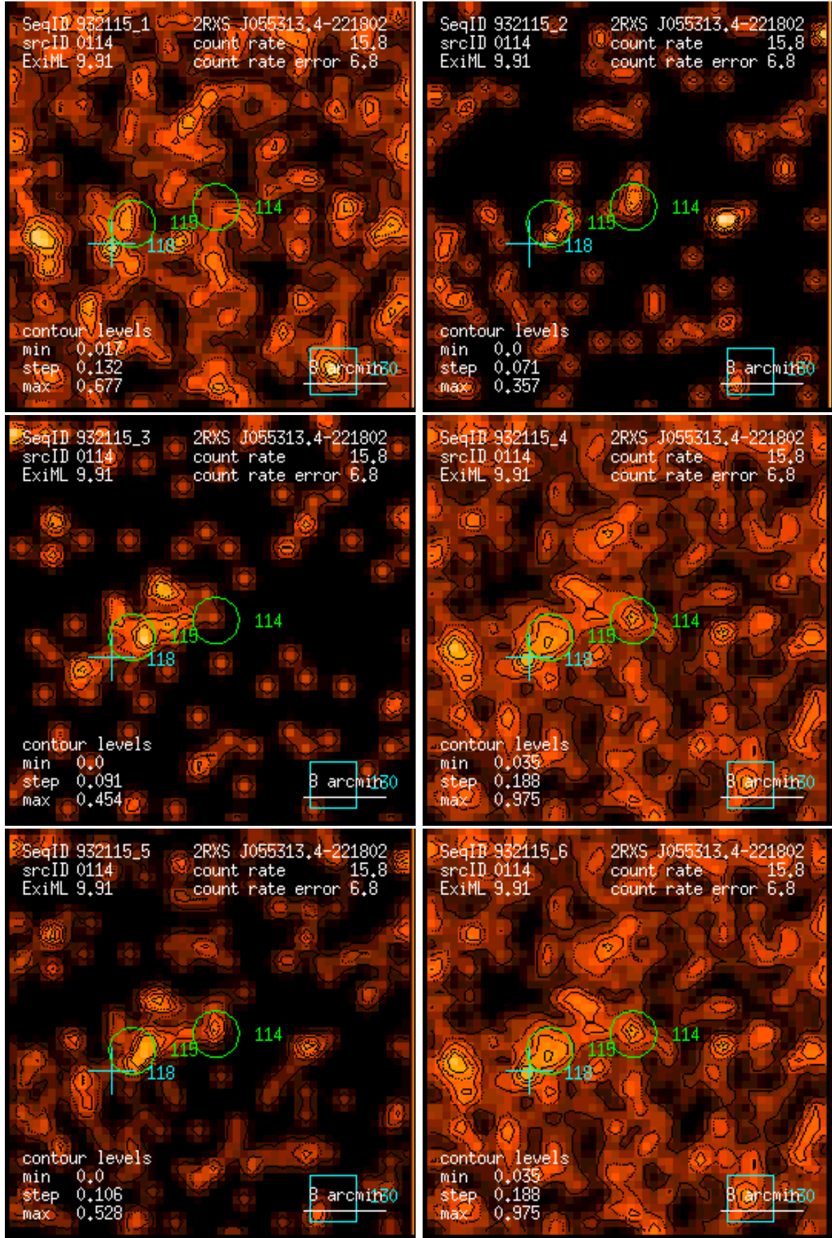
Figure 114: RASS 932115: detection 0114: band rate images, Gaussian filter: (1) PSPC channels 11 – 41, (2) 52 – 90, (3) 91 – 201, (4) 11 – 235, (5) 52 – 201, (6) 11 – 201. Broad band rates in counts/ks. Band rate contour levels in counts/ks/arcmin 2 .
