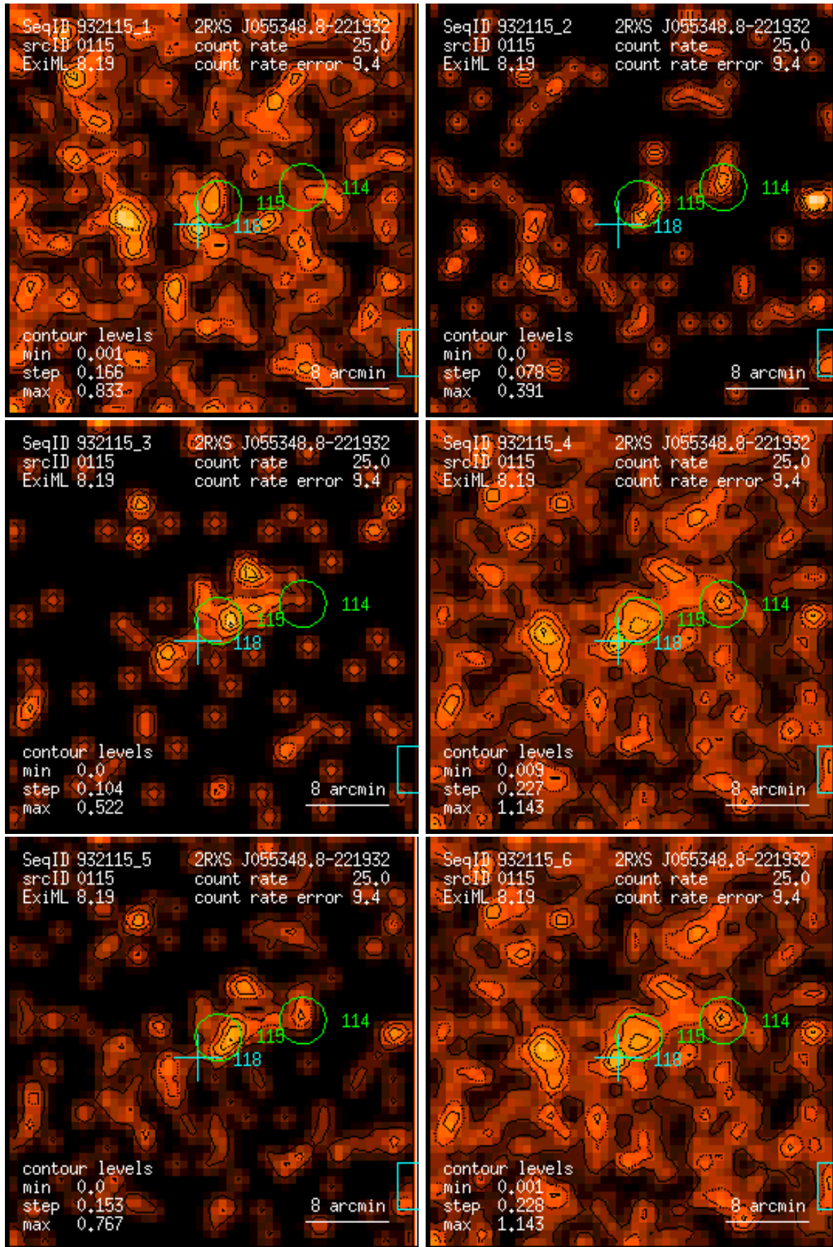
Figure 115: RASS 932115: detection 0115: band rate images, Gaussian filter: (1) PSPC channels 11 – 41, (2) 52 – 90, (3) 91 – 201, (4) 11 – 235, (5) 52 – 201, (6) 11 – 201. Broad band rates in counts/ks. Band rate contour levels in counts/ks/arcmin 2 .
