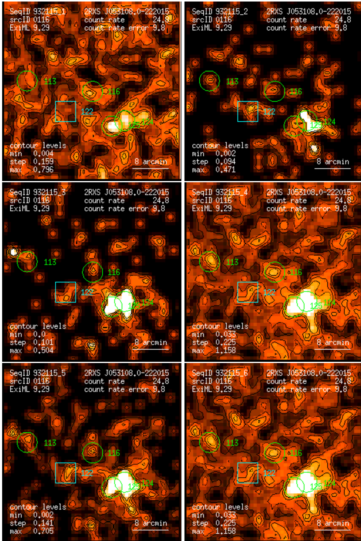
Figure 116: RASS 932115: detection 0116: band rate images, Gaussian filter: (1) PSPC channels 11 – 41, (2) 52 – 90, (3) 91 – 201, (4) 11 – 235, (5) 52 – 201, (6) 11 – 201. Broad band rates in counts/ks. Band rate contour levels in counts/ks/arcmin 2 .
