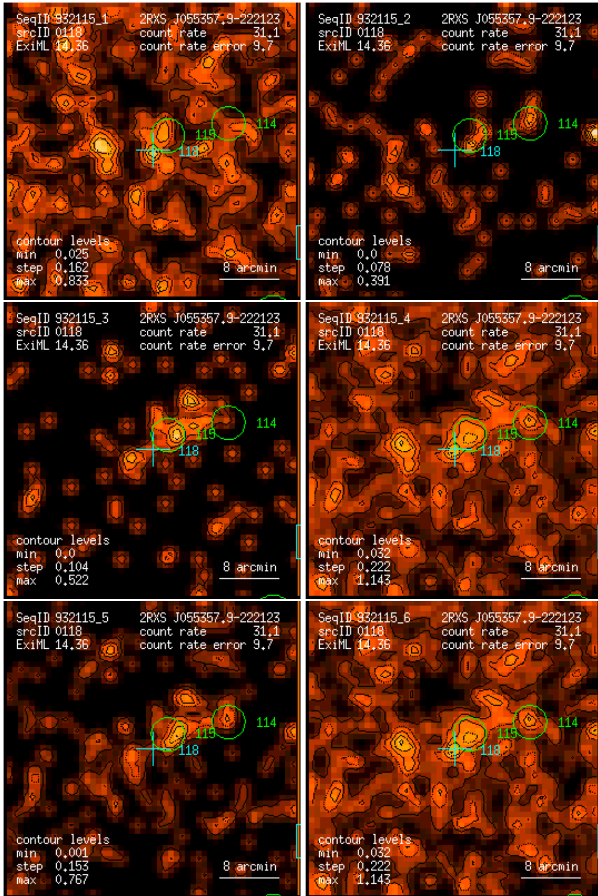
Figure 118: RASS 932115: detection 0118: band rate images, Gaussian filter: (1) PSPC channels 11 – 41, (2) 52 – 90, (3) 91 – 201, (4) 11 – 235, (5) 52 – 201, (6) 11 – 201. Broad band rates in counts/ks. Band rate contour levels in counts/ks/arcmin 2 .
