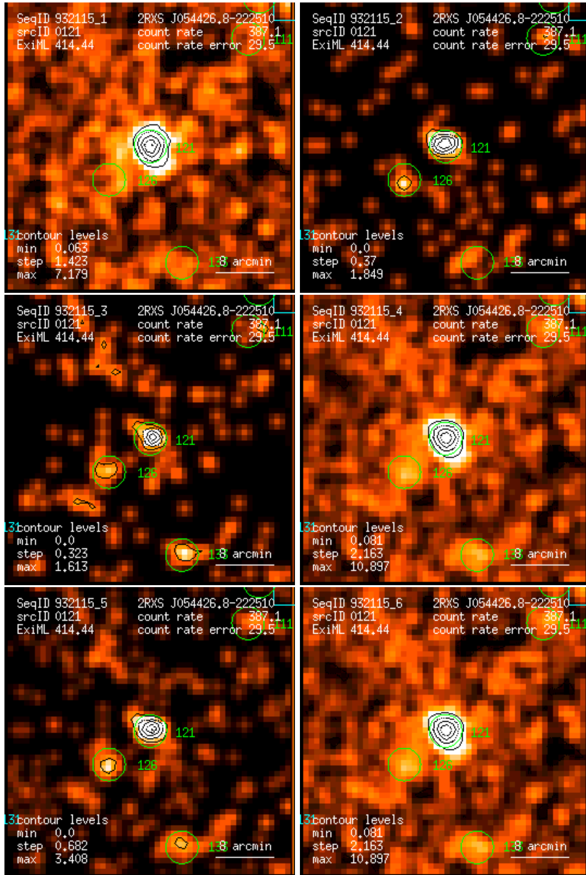
Figure 121: RASS 932115: detection 0121: band rate images, Gaussian filter: (1) PSPC channels 11 – 41, (2) 52 – 90, (3) 91 – 201, (4) 11 – 235, (5) 52 – 201, (6) 11 – 201. Broad band rates in counts/ks. Band rate contour levels in counts/ks/arcmin 2 .
