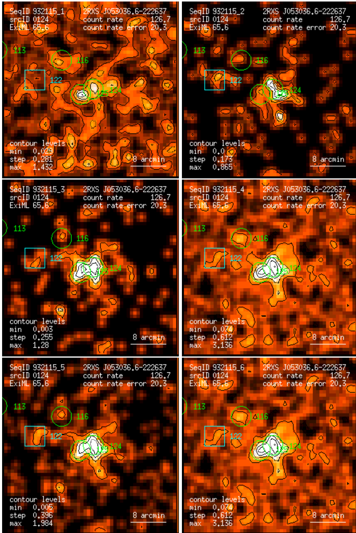
Figure 124: RASS 932115: detection 0124: band rate images, Gaussian filter: (1) PSPC channels 11 – 41, (2) 52 – 90, (3) 91 – 201, (4) 11 – 235, (5) 52 – 201, (6) 11 – 201. Broad band rates in counts/ks. Band rate contour levels in counts/ks/arcmin 2 .
