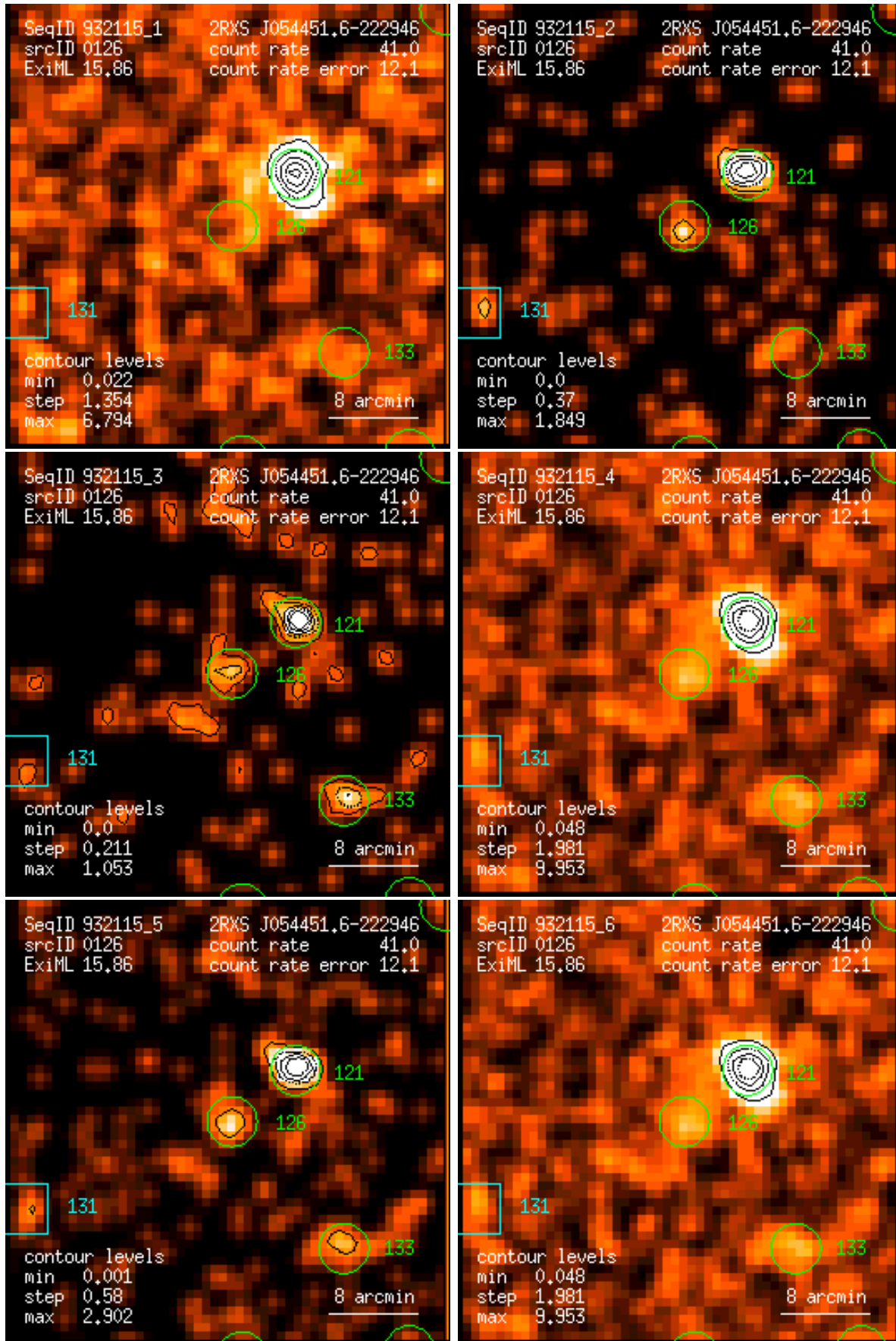
Figure 126: RASS 932115: detection 0126: band rate images, Gaussian filter: (1) PSPC channels 11 – 41, (2) 52 – 90, (3) 91 – 201, (4) 11 – 235, (5) 52 – 201, (6) 11 – 201. Broad band rates in counts/ks. Band rate contour levels in counts/ks/arcmin 2 .
