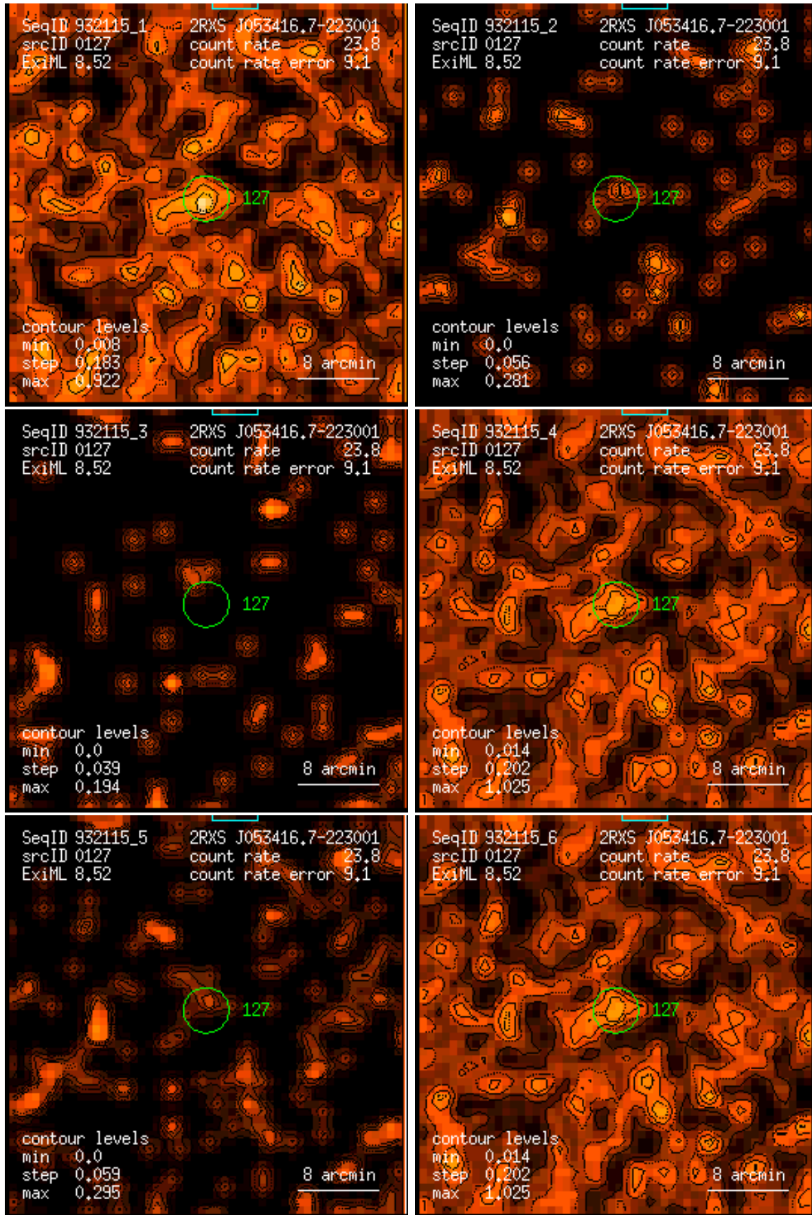
Figure 127: RASS 932115: detection 0127: band rate images, Gaussian filter: (1) PSPC channels 11 – 41, (2) 52 – 90, (3) 91 – 201, (4) 11 – 235, (5) 52 – 201, (6) 11 – 201. Broad band rates in counts/ks. Band rate contour levels in counts/ks/arcmin 2 .
