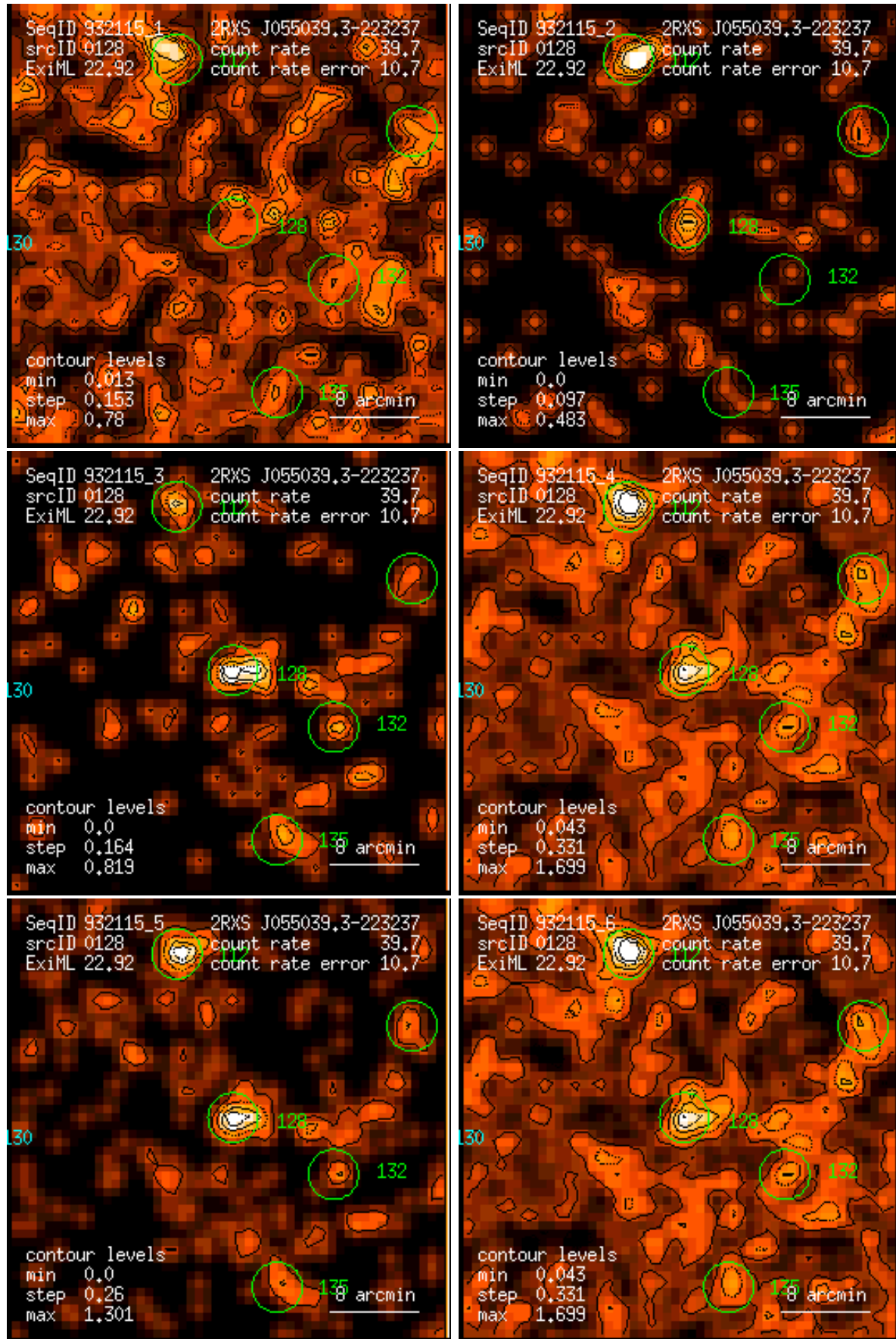
Figure 128: RASS 932115: detection 0128: band rate images, Gaussian filter: (1) PSPC channels 11 – 41, (2) 52 – 90, (3) 91 – 201, (4) 11 – 235, (5) 52 – 201, (6) 11 – 201. Broad band rates in counts/ks. Band rate contour levels in counts/ks/arcmin 2 .
