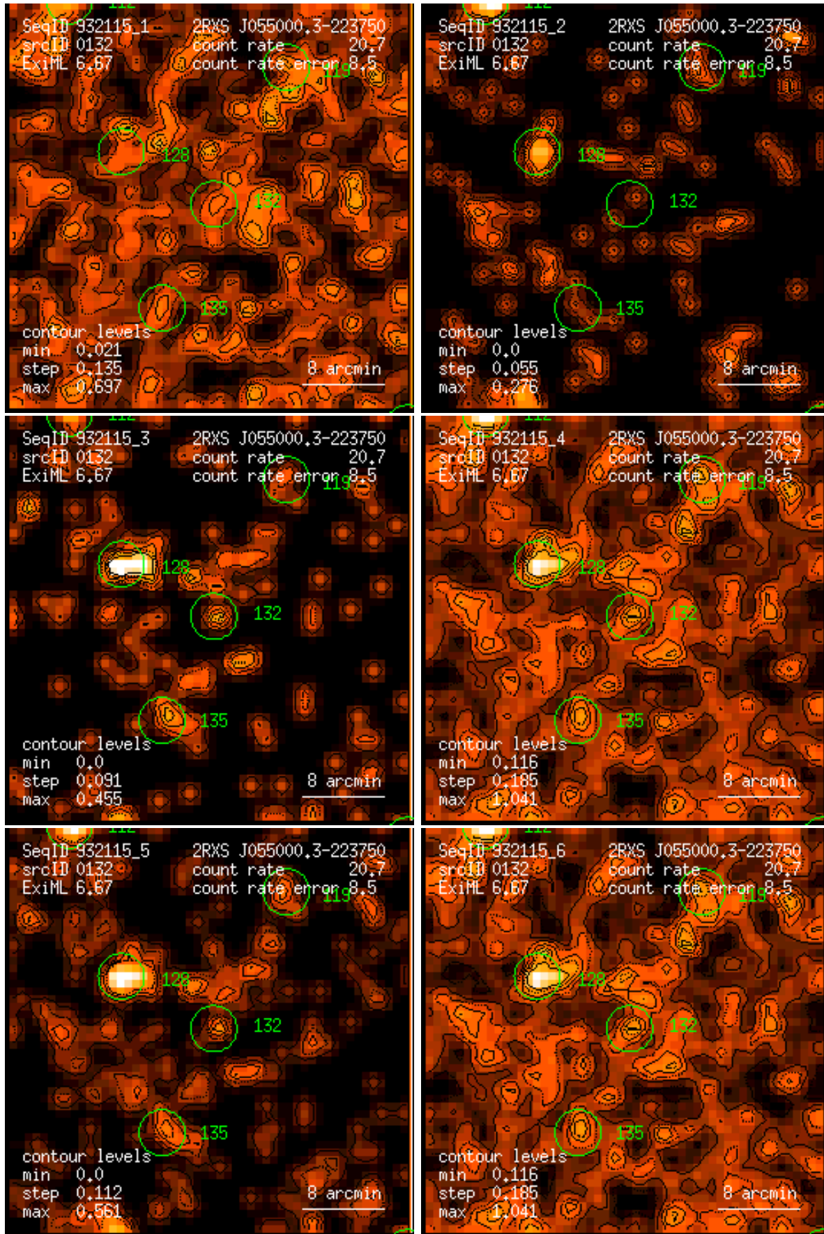
Figure 132: RASS 932115: detection 0132: band rate images, Gaussian filter: (1) PSPC channels 11 – 41, (2) 52 – 90, (3) 91 – 201, (4) 11 – 235, (5) 52 – 201, (6) 11 – 201. Broad band rates in counts/ks. Band rate contour levels in counts/ks/arcmin 2 .
