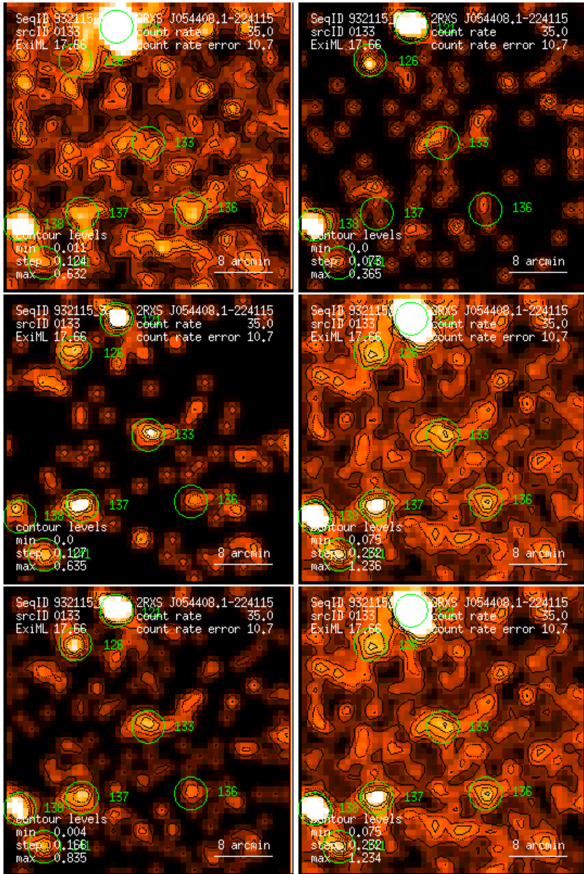
Figure 133: RASS 932115: detection 0133: band rate images, Gaussian filter: (1) PSPC channels 11 – 41, (2) 52 – 90, (3) 91 – 201, (4) 11 – 235, (5) 52 – 201, (6) 11 – 201. Broad band rates in counts/ks. Band rate contour levels in counts/ks/arcmin 2 .
