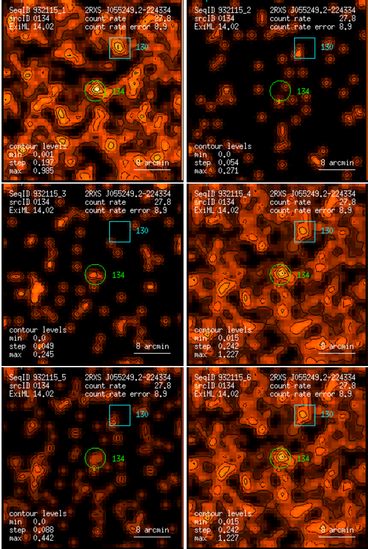
Figure 134: RASS 932115: detection 0134: band rate images, Gaussian filter: (1) PSPC channels 11 – 41, (2) 52 – 90, (3) 91 – 201, (4) 11 – 235, (5) 52 – 201, (6) 11 – 201. Broad band rates in counts/ks. Band rate contour levels in counts/ks/arcmin 2 .
