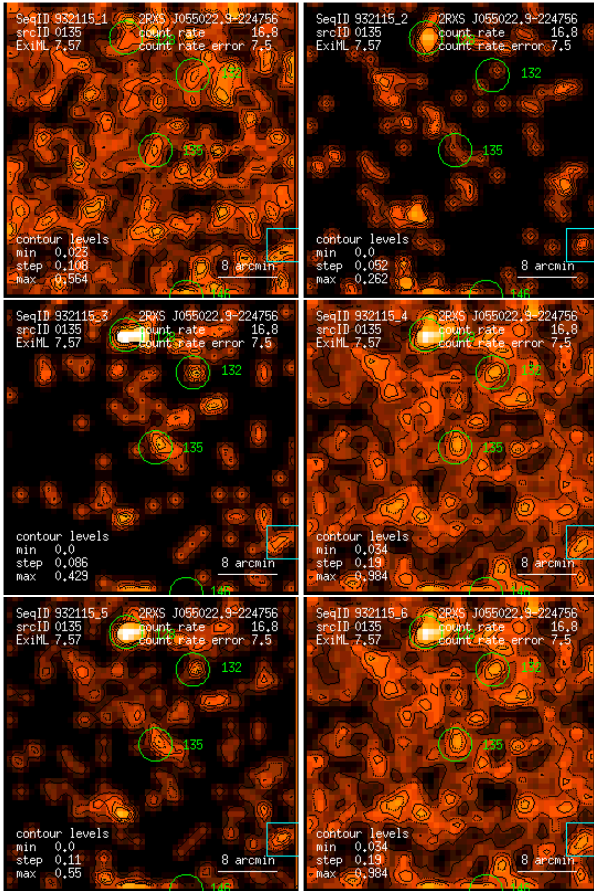
Figure 135: RASS 932115: detection 0135: band rate images, Gaussian filter: (1) PSPC channels 11 – 41, (2) 52 – 90, (3) 91 – 201, (4) 11 – 235, (5) 52 – 201, (6) 11 – 201. Broad band rates in counts/ks. Band rate contour levels in counts/ks/arcmin 2 .
