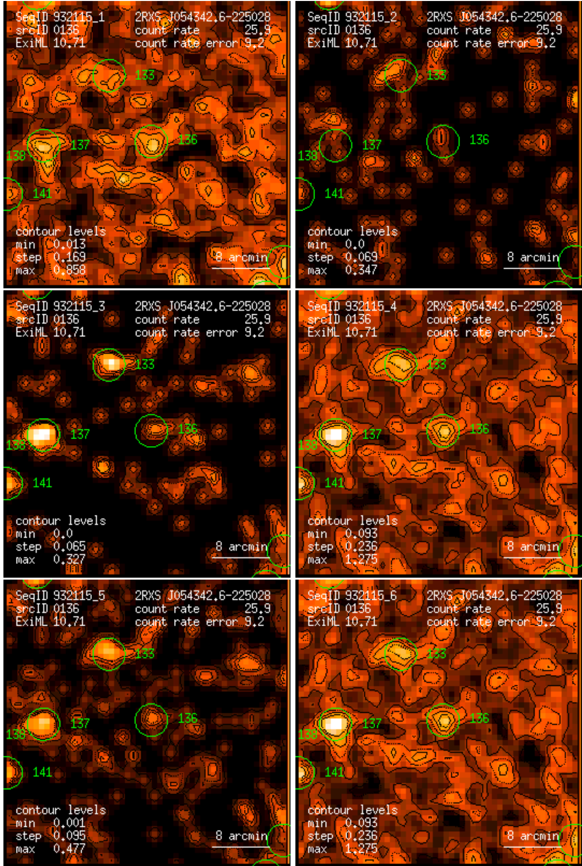
Figure 136: RASS 932115: detection 0136: band rate images, Gaussian filter: (1) PSPC channels 11 – 41, (2) 52 – 90, (3) 91 – 201, (4) 11 – 235, (5) 52 – 201, (6) 11 – 201. Broad band rates in counts/ks. Band rate contour levels in counts/ks/arcmin 2 .
