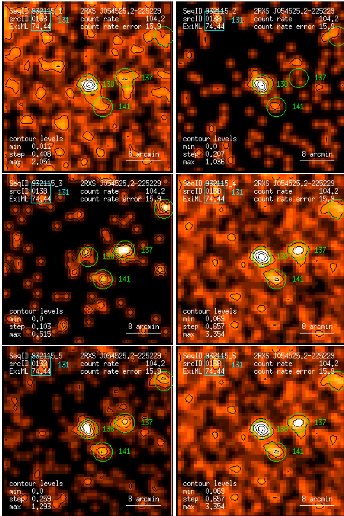
Figure 138: RASS 932115: detection 0138: band rate images, Gaussian filter: (1) PSPC channels 11 – 41, (2) 52 – 90, (3) 91 – 201, (4) 11 – 235, (5) 52 – 201, (6) 11 – 201. Broad band rates in counts/ks. Band rate contour levels in counts/ks/arcmin 2 .
