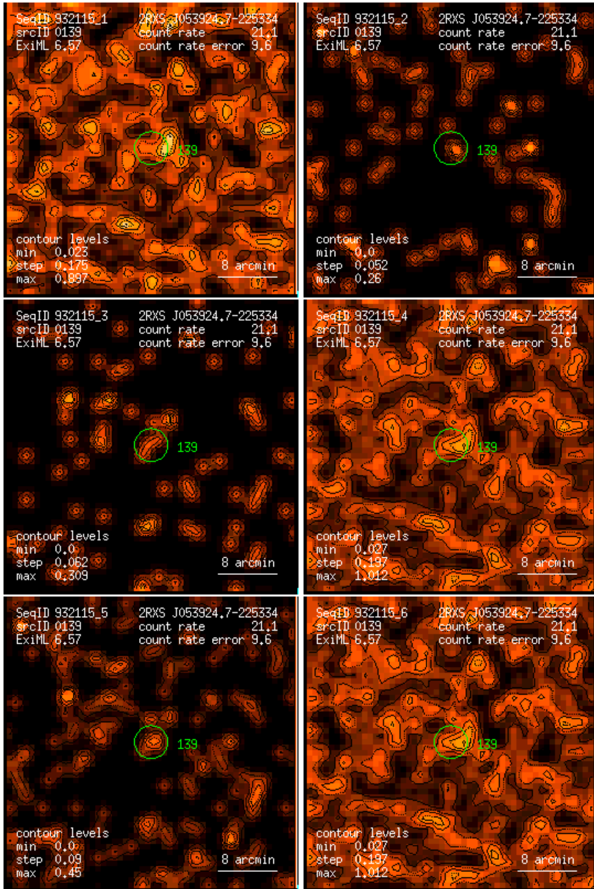
Figure 139: RASS 932115: detection 0139: band rate images, Gaussian filter: (1) PSPC channels 11 – 41, (2) 52 – 90, (3) 91 – 201, (4) 11 – 235, (5) 52 – 201, (6) 11 – 201. Broad band rates in counts/ks. Band rate contour levels in counts/ks/arcmin 2 .
