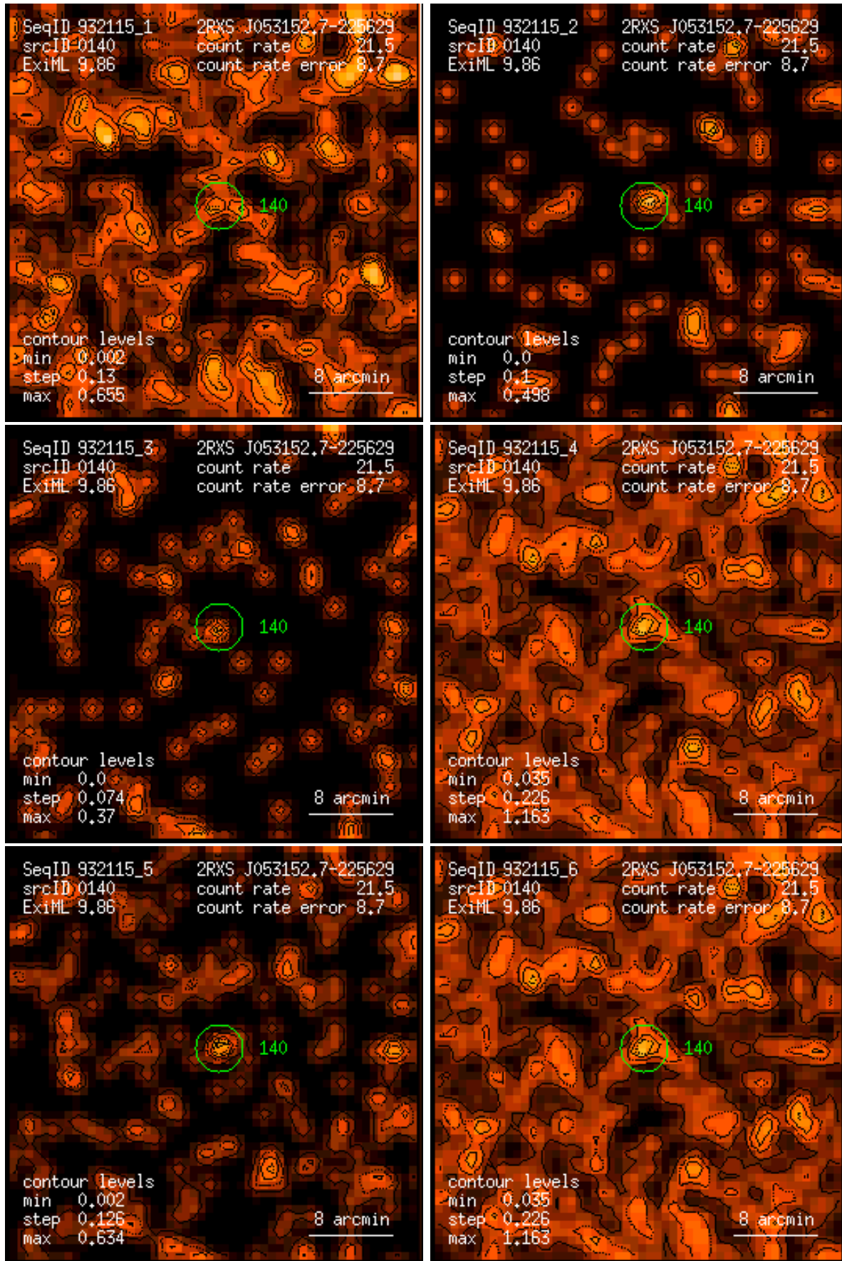
Figure 140: RASS 932115: detection 0140: band rate images, Gaussian filter: (1) PSPC channels 11 – 41, (2) 52 – 90, (3) 91 – 201, (4) 11 – 235, (5) 52 – 201, (6) 11 – 201. Broad band rates in counts/ks. Band rate contour levels in counts/ks/arcmin 2 .
