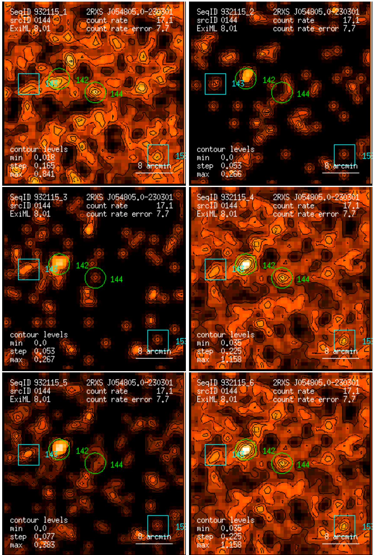
Figure 144: RASS 932115: detection 0144: band rate images, Gaussian filter: (1) PSPC channels 11 – 41, (2) 52 – 90, (3) 91 – 201, (4) 11 – 235, (5) 52 – 201, (6) 11 – 201. Broad band rates in counts/ks. Band rate contour levels in counts/ks/arcmin 2 .
