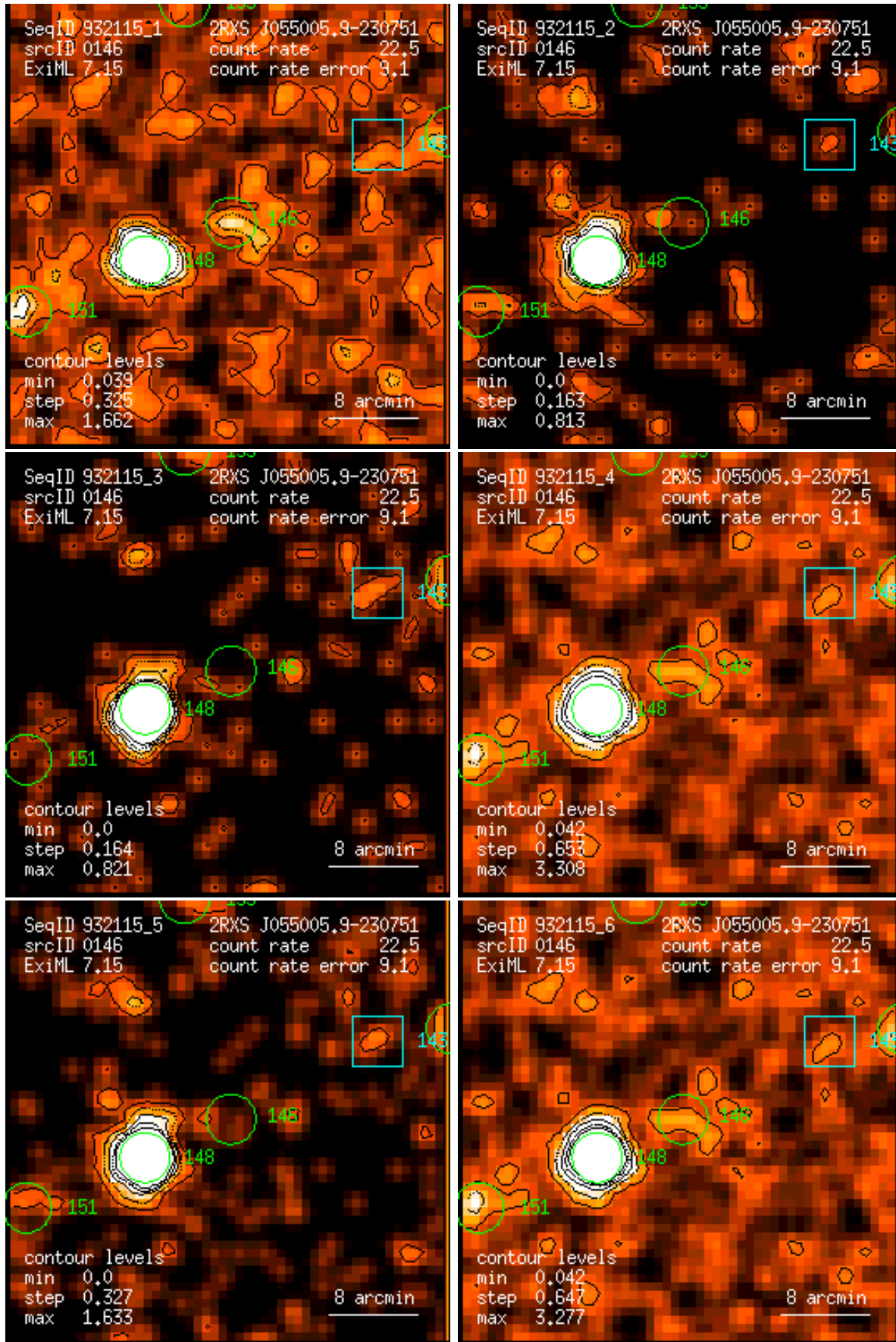
Figure 146: RASS 932115: detection 0146: band rate images, Gaussian filter: (1) PSPC channels 11 – 41, (2) 52 – 90, (3) 91 – 201, (4) 11 – 235, (5) 52 – 201, (6) 11 – 201. Broad band rates in counts/ks. Band rate contour levels in counts/ks/arcmin 2 .
