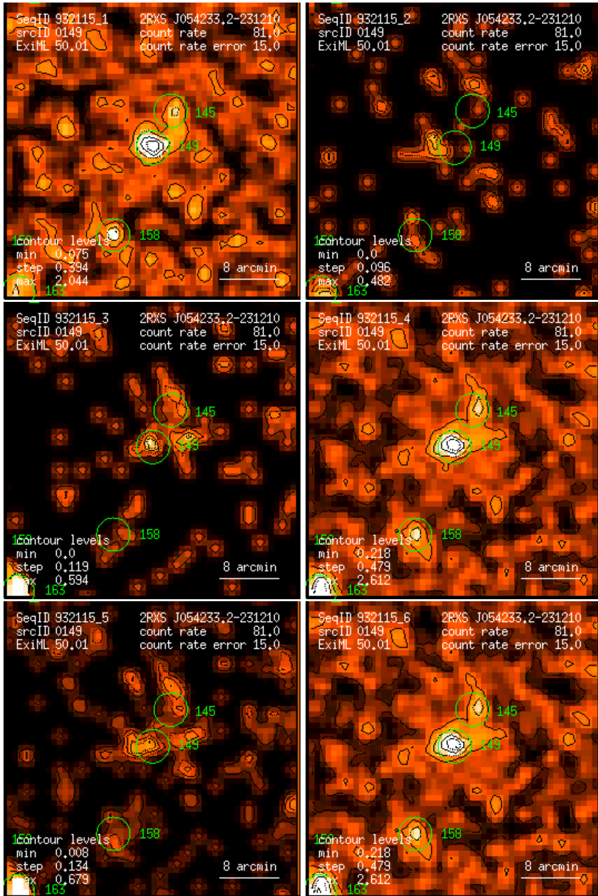
Figure 149: RASS 932115: detection 0149: band rate images, Gaussian filter: (1) PSPC channels 11 – 41, (2) 52 – 90, (3) 91 – 201, (4) 11 – 235, (5) 52 – 201, (6) 11 – 201. Broad band rates in counts/ks. Band rate contour levels in counts/ks/arcmin 2 .
