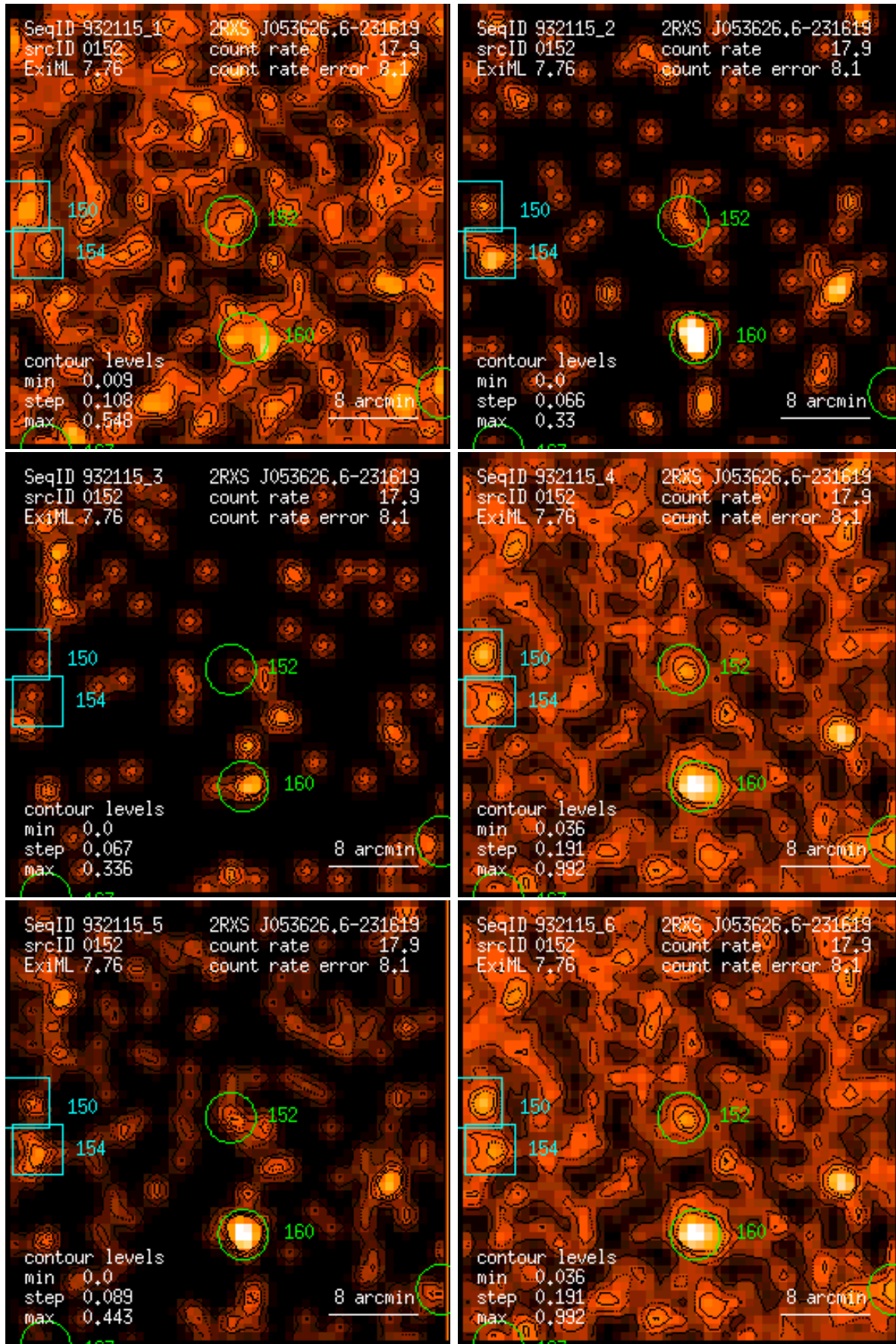
Figure 152: RASS 932115: detection 0152: band rate images, Gaussian filter: (1) PSPC channels 11 – 41, (2) 52 – 90, (3) 91 – 201, (4) 11 – 235, (5) 52 – 201, (6) 11 – 201. Broad band rates in counts/ks. Band rate contour levels in counts/ks/arcmin 2 .
