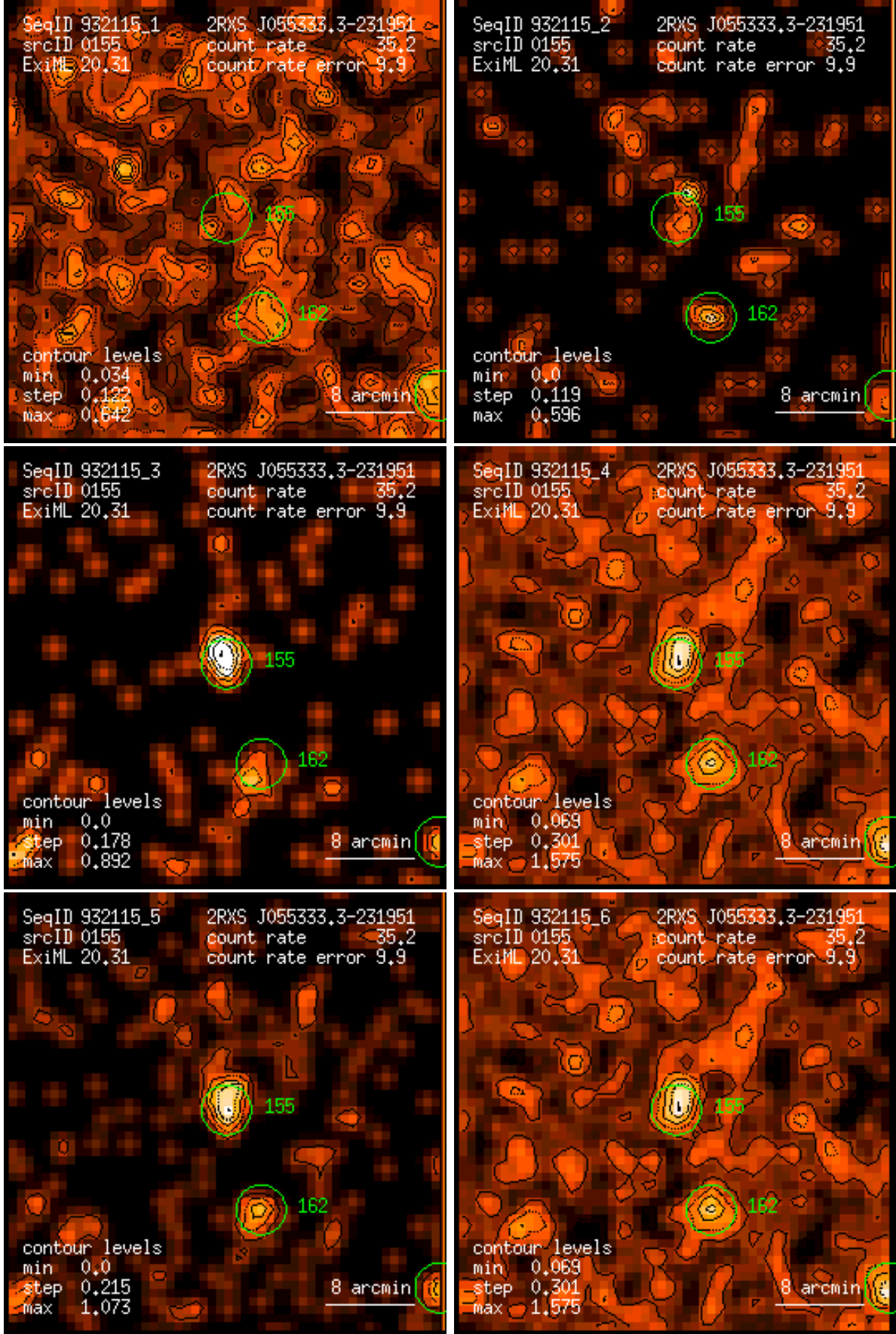
Figure 155: RASS 932115: detection 0155: band rate images, Gaussian filter: (1) PSPC channels 11 – 41, (2) 52 – 90, (3) 91 – 201, (4) 11 – 235, (5) 52 – 201, (6) 11 – 201. Broad band rates in counts/ks. Band rate contour levels in counts/ks/arcmin 2 .
