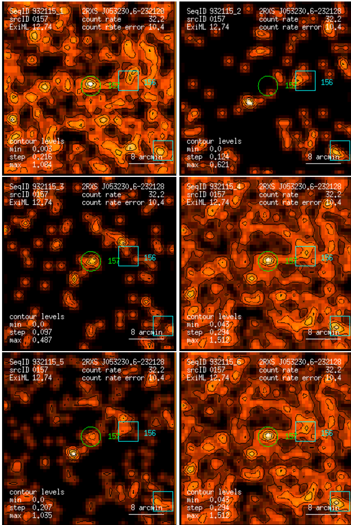
Figure 157: RASS 932115: detection 0157: band rate images, Gaussian filter: (1) PSPC channels 11 – 41, (2) 52 – 90, (3) 91 – 201, (4) 11 – 235, (5) 52 – 201, (6) 11 – 201. Broad band rates in counts/ks. Band rate contour levels in counts/ks/arcmin 2 .
